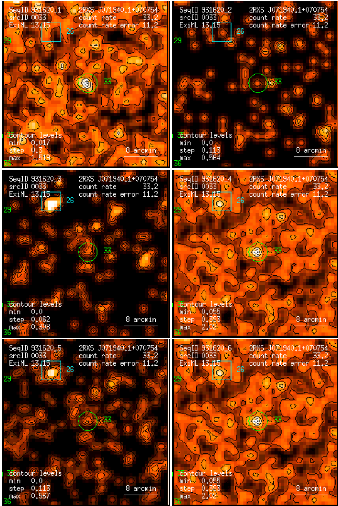
Figure 33: RASS 931620: detection 0033: band rate images, Gaussian filter: (1) PSPC channels 11 – 41, (2) 52 – 90, (3) 91 – 201, (4) 11 – 235, (5) 52 – 201, (6) 11 – 201. Broad band rates in counts/ks. Band rate contour levels in counts/ks/arcmin 2 .
