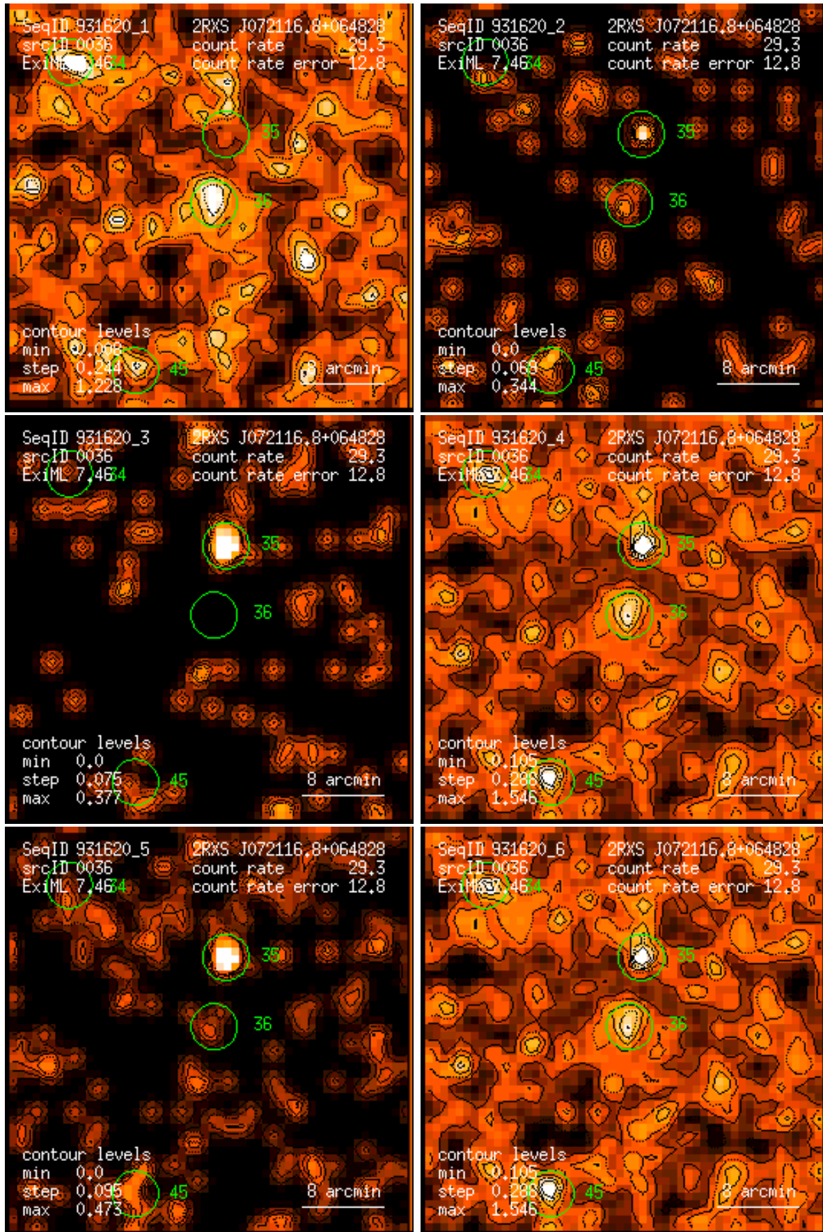
Figure 36: RASS 931620: detection 0036: band rate images, Gaussian filter: (1) PSPC channels 11 – 41, (2) 52 – 90, (3) 91 – 201, (4) 11 – 235, (5) 52 – 201, (6) 11 – 201. Broad band rates in counts/ks. Band rate contour levels in counts/ks/arcmin 2 .
