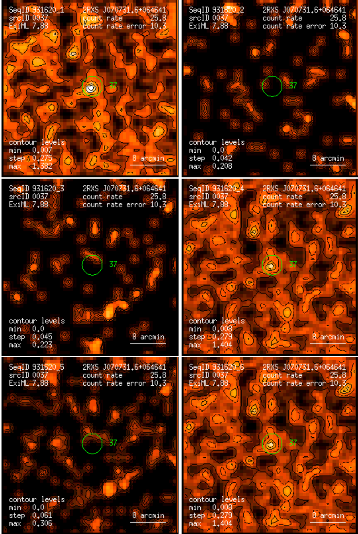
Figure 37: RASS 931620: detection 0037: band rate images, Gaussian filter: (1) PSPC channels 11 – 41, (2) 52 – 90, (3) 91 – 201, (4) 11 – 235, (5) 52 – 201, (6) 11 – 201. Broad band rates in counts/ks. Band rate contour levels in counts/ks/arcmin 2 .
