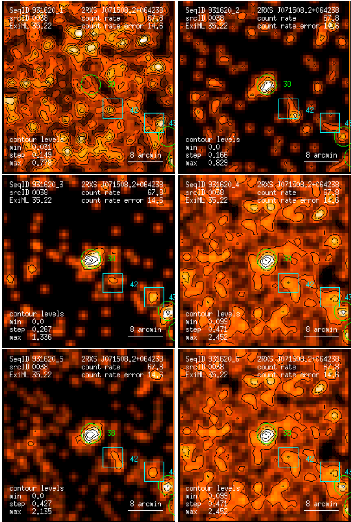
Figure 38: RASS 931620: detection 0038: band rate images, Gaussian filter: (1) PSPC channels 11 – 41, (2) 52 – 90, (3) 91 – 201, (4) 11 – 235, (5) 52 – 201, (6) 11 – 201. Broad band rates in counts/ks. Band rate contour levels in counts/ks/arcmin 2 .
