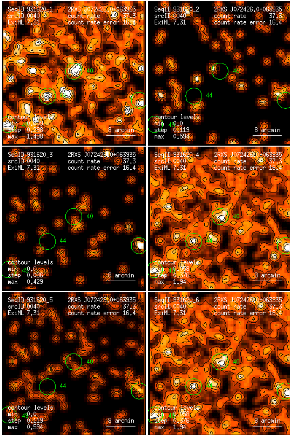
Figure 40: RASS 931620: detection 0040: band rate images, Gaussian filter: (1) PSPC channels 11 – 41, (2) 52 – 90, (3) 91 – 201, (4) 11 – 235, (5) 52 – 201, (6) 11 – 201. Broad band rates in counts/ks. Band rate contour levels in counts/ks/arcmin 2 .
