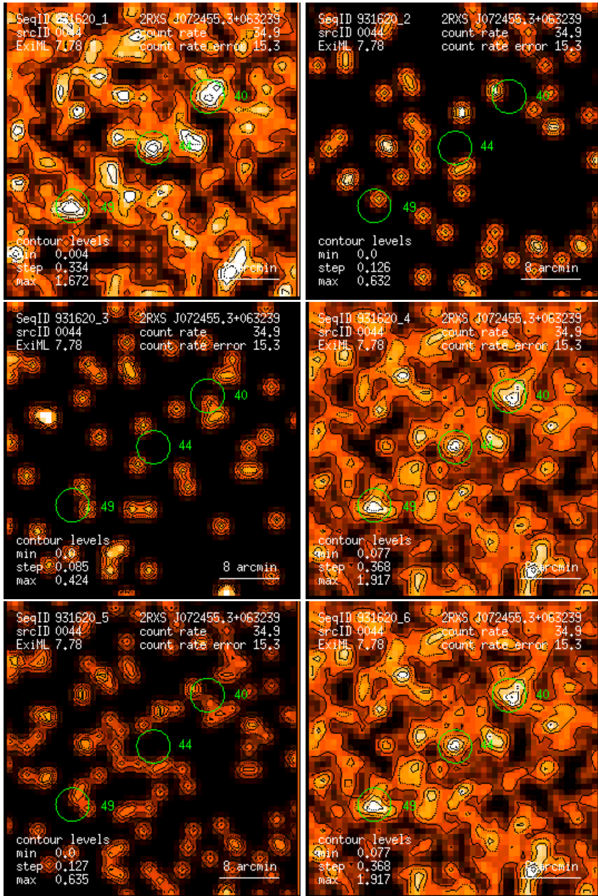
Figure 44: RASS 931620: detection 0044: band rate images, Gaussian filter: (1) PSPC channels 11 – 41, (2) 52 – 90, (3) 91 – 201, (4) 11 – 235, (5) 52 – 201, (6) 11 – 201. Broad band rates in counts/ks. Band rate contour levels in counts/ks/arcmin 2 .
