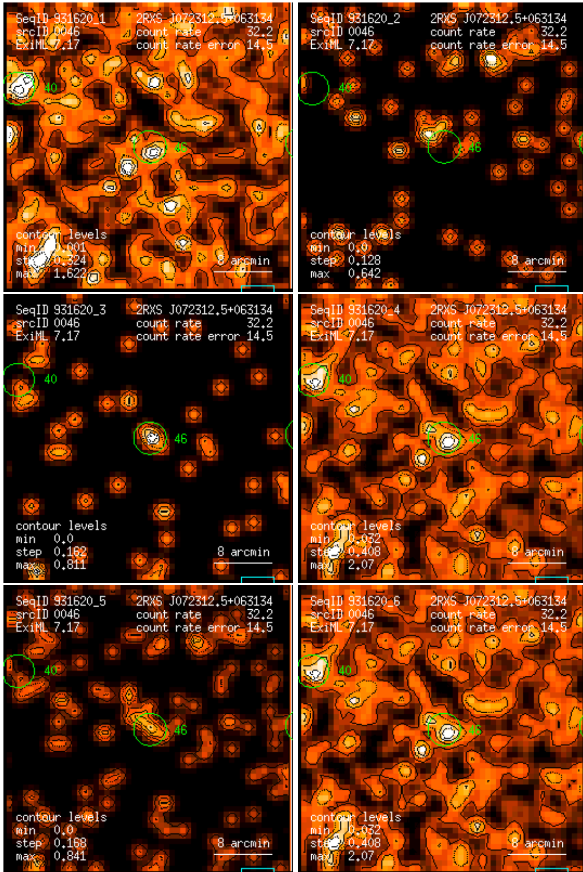
Figure 46: RASS 931620: detection 0046: band rate images, Gaussian filter: (1) PSPC channels 11 – 41, (2) 52 – 90, (3) 91 – 201, (4) 11 – 235, (5) 52 – 201, (6) 11 – 201. Broad band rates in counts/ks. Band rate contour levels in counts/ks/arcmin 2 .
