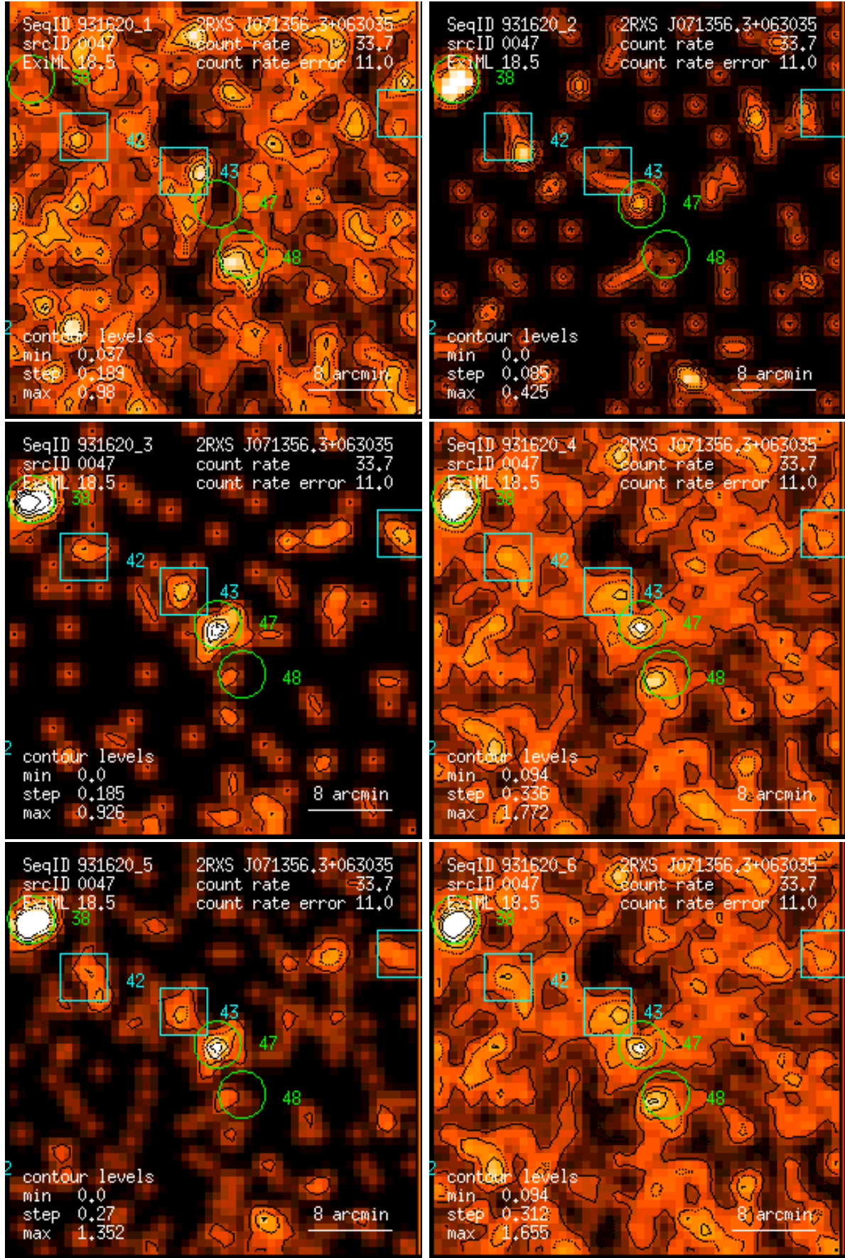
Figure 47: RASS 931620: detection 0047: band rate images, Gaussian filter: (1) PSPC channels 11 – 41, (2) 52 – 90, (3) 91 – 201, (4) 11 – 235, (5) 52 – 201, (6) 11 – 201. Broad band rates in counts/ks. Band rate contour levels in counts/ks/arcmin 2 .
