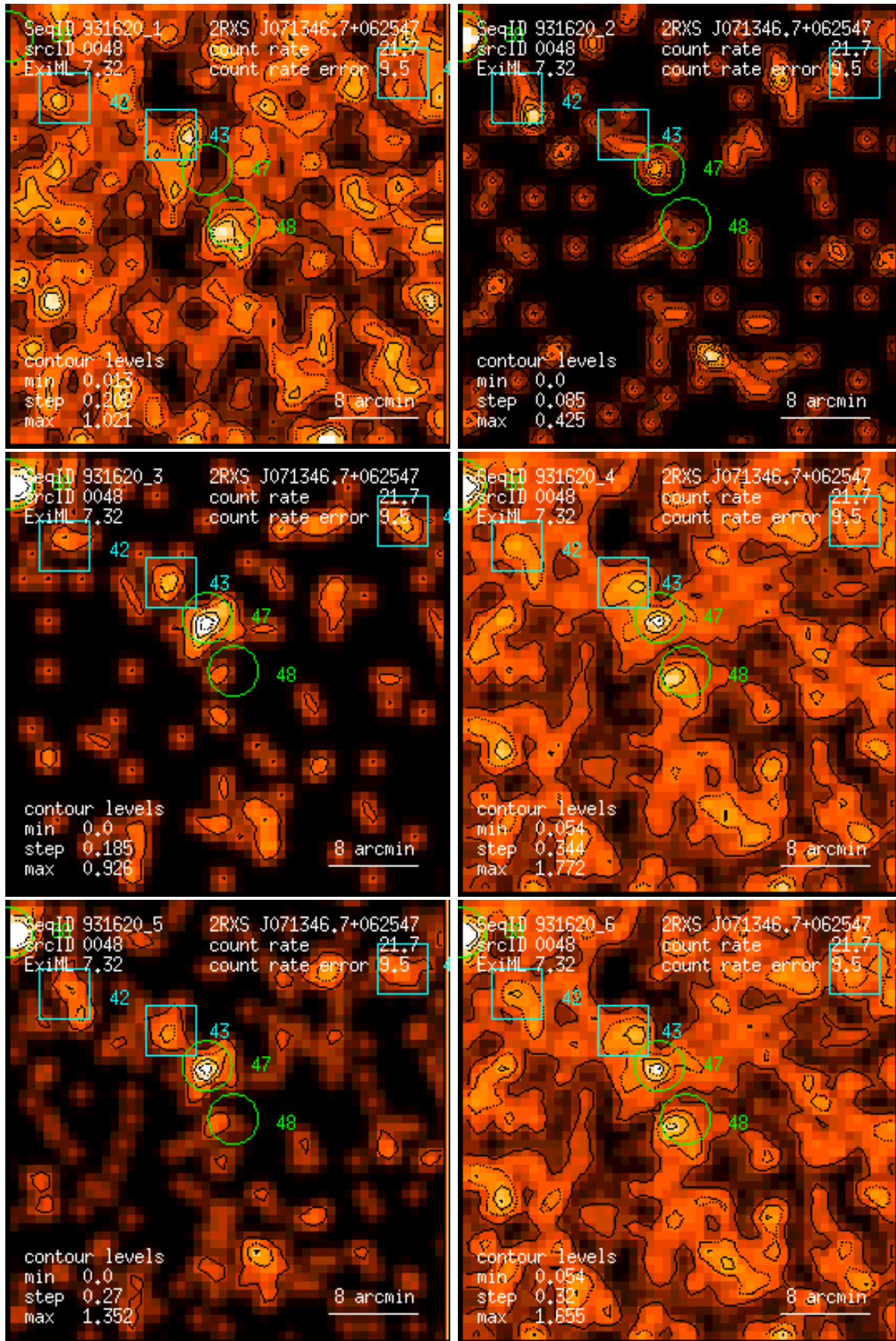
Figure 48: RASS 931620: detection 0048: band rate images, Gaussian filter: (1) PSPC channels 11 – 41, (2) 52 – 90, (3) 91 – 201, (4) 11 – 235, (5) 52 – 201, (6) 11 – 201. Broad band rates in counts/ks. Band rate contour levels in counts/ks/arcmin 2 .
