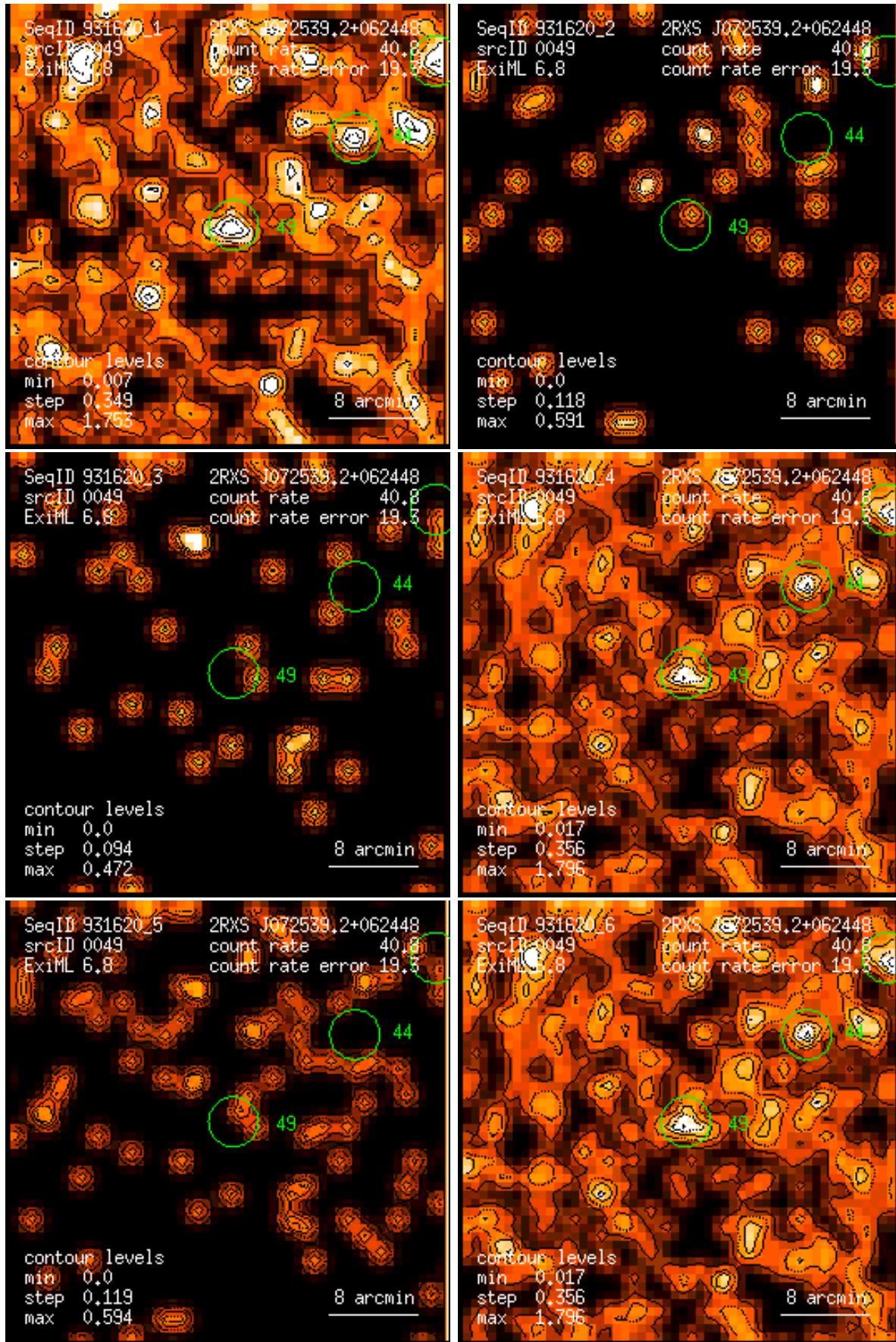
Figure 49: RASS 931620: detection 0049: band rate images, Gaussian filter: (1) PSPC channels 11 – 41, (2) 52 – 90, (3) 91 – 201, (4) 11 – 235, (5) 52 – 201, (6) 11 – 201. Broad band rates in counts/ks. Band rate contour levels in counts/ks/arcmin 2 .
