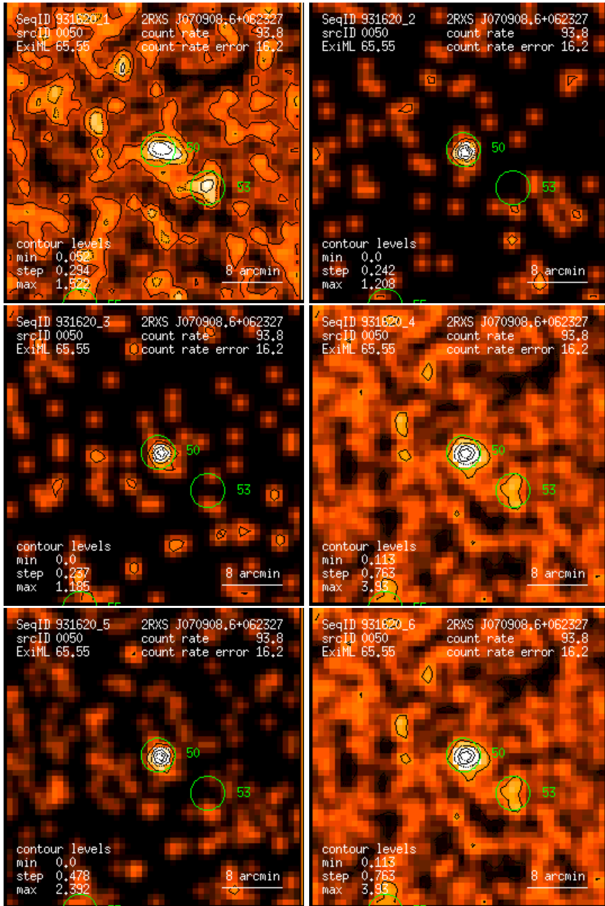
Figure 50: RASS 931620: detection 0050: band rate images, Gaussian filter: (1) PSPC channels 11 – 41, (2) 52 – 90, (3) 91 – 201, (4) 11 – 235, (5) 52 – 201, (6) 11 – 201. Broad band rates in counts/ks. Band rate contour levels in counts/ks/arcmin 2 .
