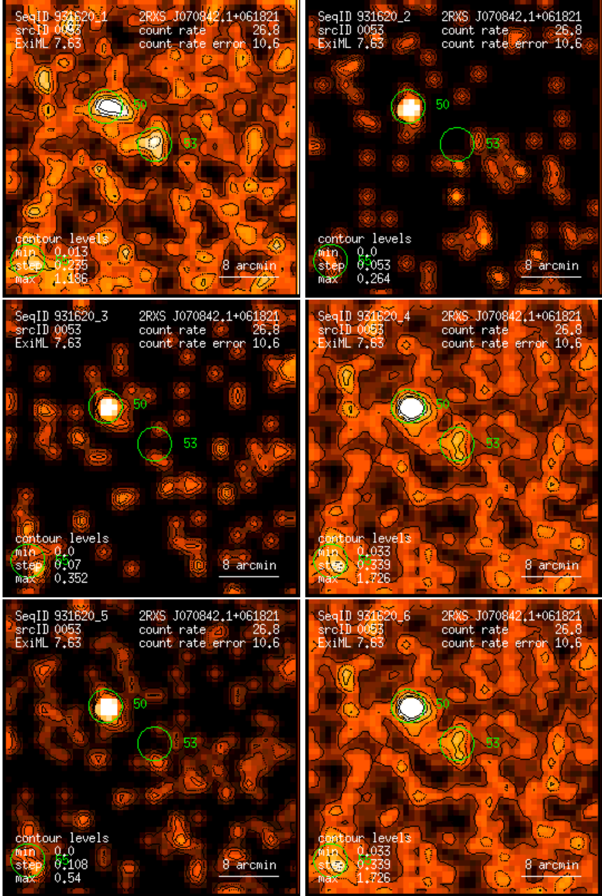
Figure 53: RASS 931620: detection 0053: band rate images, Gaussian filter: (1) PSPC channels 11 – 41, (2) 52 – 90, (3) 91 – 201, (4) 11 – 235, (5) 52 – 201, (6) 11 – 201. Broad band rates in counts/ks. Band rate contour levels in counts/ks/arcmin 2 .
