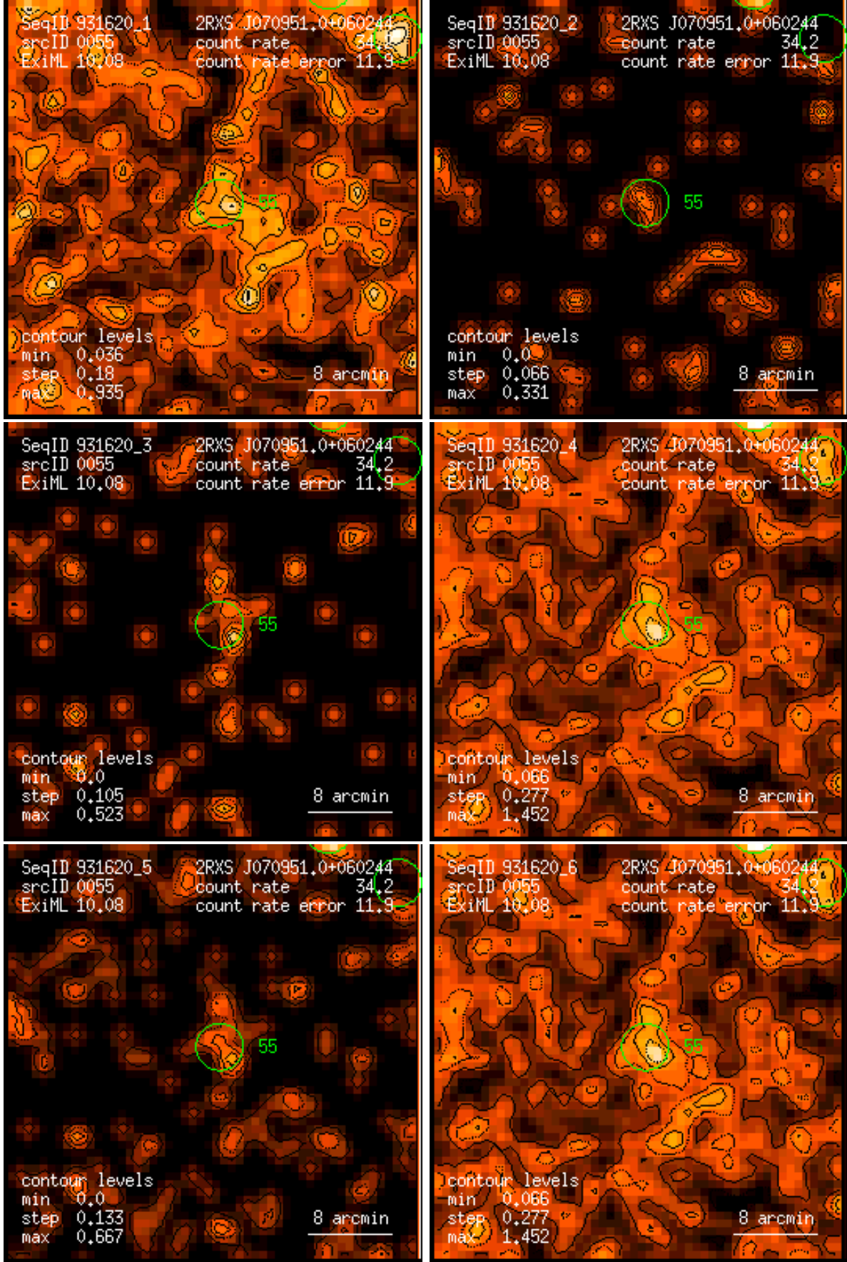
Figure 55: RASS 931620: detection 0055: band rate images, Gaussian filter: (1) PSPC channels 11 – 41, (2) 52 – 90, (3) 91 – 201, (4) 11 – 235, (5) 52 – 201, (6) 11 – 201. Broad band rates in counts/ks. Band rate contour levels in counts/ks/arcmin 2 .
