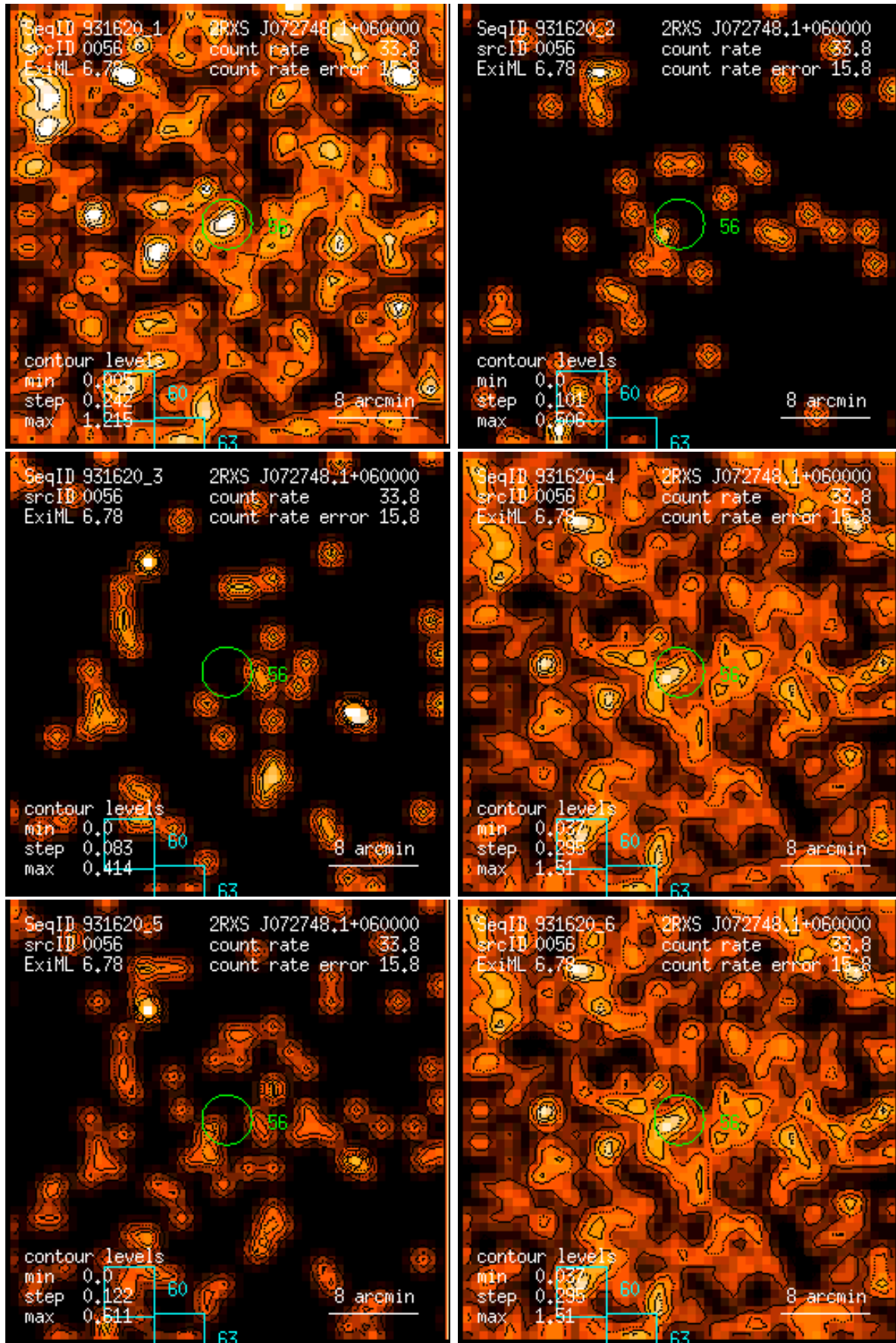
Figure 56: RASS 931620: detection 0056: band rate images, Gaussian filter: (1) PSPC channels 11 – 41, (2) 52 – 90, (3) 91 – 201, (4) 11 – 235, (5) 52 – 201, (6) 11 – 201. Broad band rates in counts/ks. Band rate contour levels in counts/ks/arcmin 2 .
