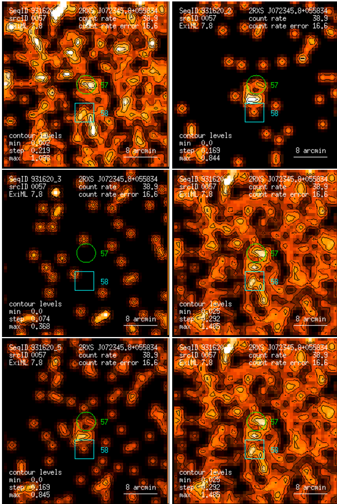
Figure 57: RASS 931620: detection 0057: band rate images, Gaussian filter: (1) PSPC channels 11 – 41, (2) 52 – 90, (3) 91 – 201, (4) 11 – 235, (5) 52 – 201, (6) 11 – 201. Broad band rates in counts/ks. Band rate contour levels in counts/ks/arcmin 2 .
