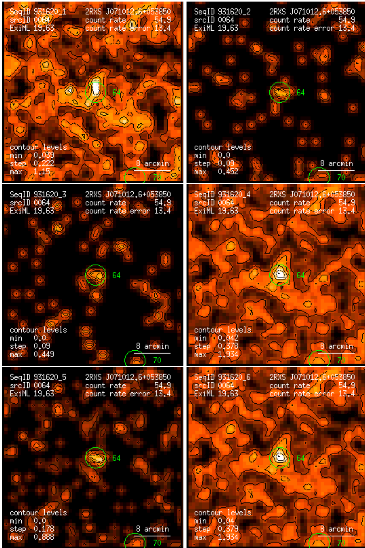
Figure 64: RASS 931620: detection 0064: band rate images, Gaussian filter: (1) PSPC channels 11 – 41, (2) 52 – 90, (3) 91 – 201, (4) 11 – 235, (5) 52 – 201, (6) 11 – 201. Broad band rates in counts/ks. Band rate contour levels in counts/ks/arcmin 2 .
