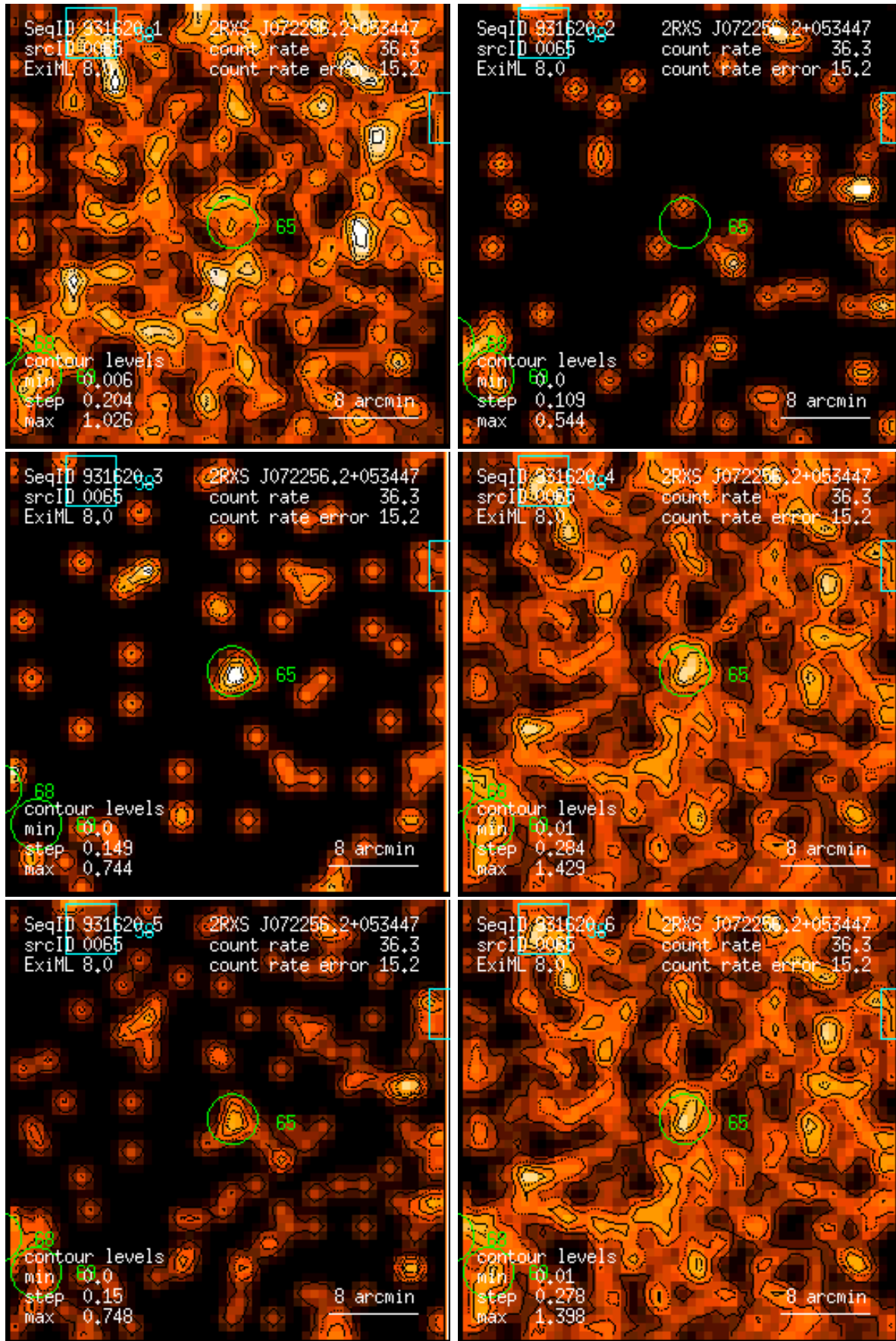
Figure 65: RASS 931620: detection 0065: band rate images, Gaussian filter: (1) PSPC channels 11 – 41, (2) 52 – 90, (3) 91 – 201, (4) 11 – 235, (5) 52 – 201, (6) 11 – 201. Broad band rates in counts/ks. Band rate contour levels in counts/ks/arcmin 2 .
