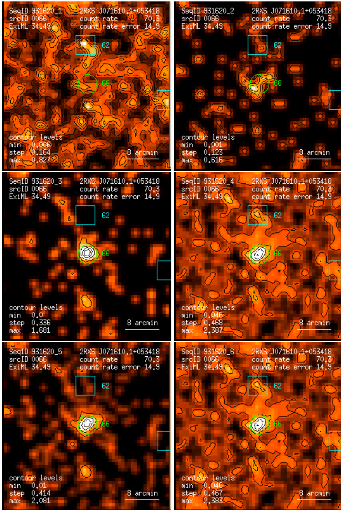
Figure 66: RASS 931620: detection 0066: band rate images, Gaussian filter: (1) PSPC channels 11 – 41, (2) 52 – 90, (3) 91 – 201, (4) 11 – 235, (5) 52 – 201, (6) 11 – 201. Broad band rates in counts/ks. Band rate contour levels in counts/ks/arcmin 2 .
