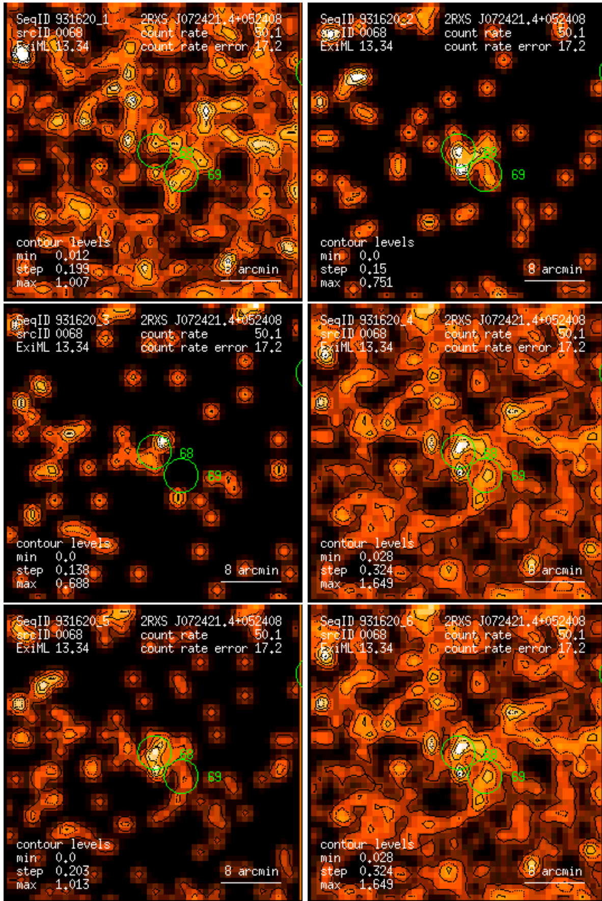
Figure 68: RASS 931620: detection 0068: band rate images, Gaussian filter: (1) PSPC channels 11 – 41, (2) 52 – 90, (3) 91 – 201, (4) 11 – 235, (5) 52 – 201, (6) 11 – 201. Broad band rates in counts/ks. Band rate contour levels in counts/ks/arcmin 2 .
