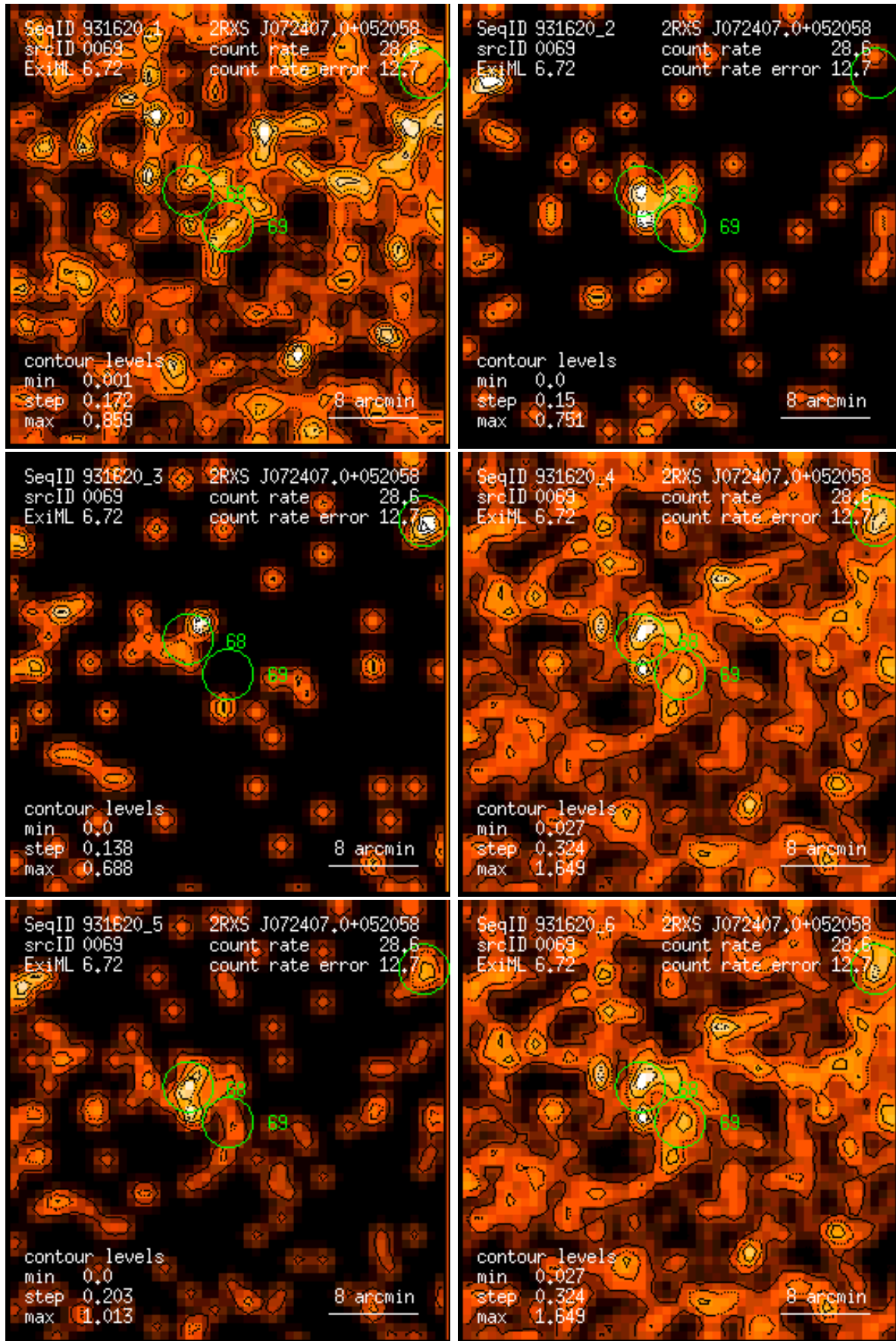
Figure 69: RASS 931620: detection 0069: band rate images, Gaussian filter: (1) PSPC channels 11 – 41, (2) 52 – 90, (3) 91 – 201, (4) 11 – 235, (5) 52 – 201, (6) 11 – 201. Broad band rates in counts/ks. Band rate contour levels in counts/ks/arcmin 2 .
