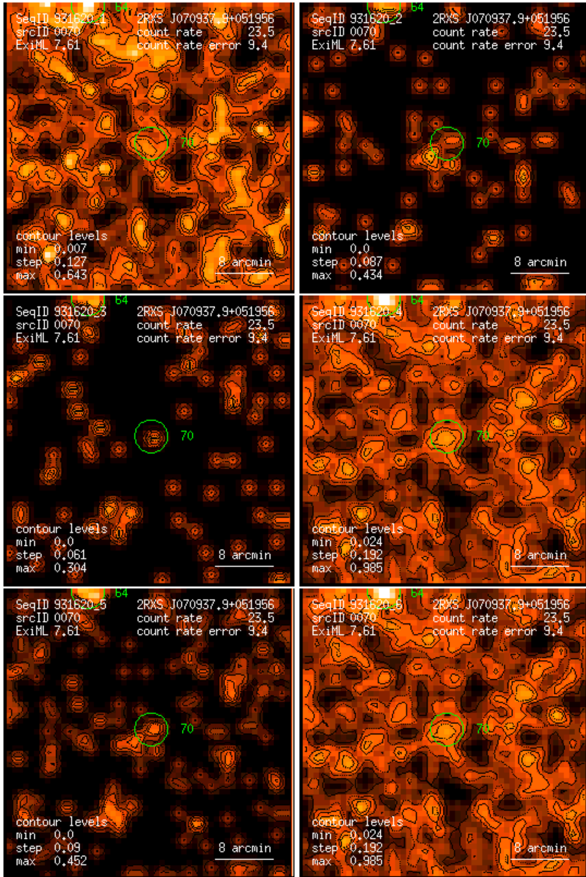
Figure 70: RASS 931620: detection 0070: band rate images, Gaussian filter: (1) PSPC channels 11 – 41, (2) 52 – 90, (3) 91 – 201, (4) 11 – 235, (5) 52 – 201, (6) 11 – 201. Broad band rates in counts/ks. Band rate contour levels in counts/ks/arcmin 2 .
