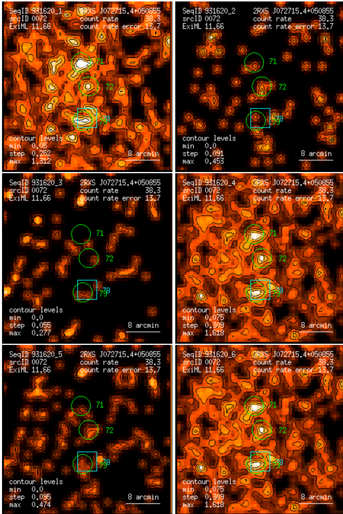
Figure 72: RASS 931620: detection 0072: band rate images, Gaussian filter: (1) PSPC channels 11 – 41, (2) 52 – 90, (3) 91 – 201, (4) 11 – 235, (5) 52 – 201, (6) 11 – 201. Broad band rates in counts/ks. Band rate contour levels in counts/ks/arcmin 2 .
