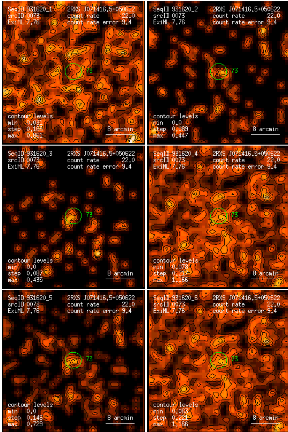
Figure 73: RASS 931620: detection 0073: band rate images, Gaussian filter: (1) PSPC channels 11 – 41, (2) 52 – 90, (3) 91 – 201, (4) 11 – 235, (5) 52 – 201, (6) 11 – 201. Broad band rates in counts/ks. Band rate contour levels in counts/ks/arcmin 2 .
