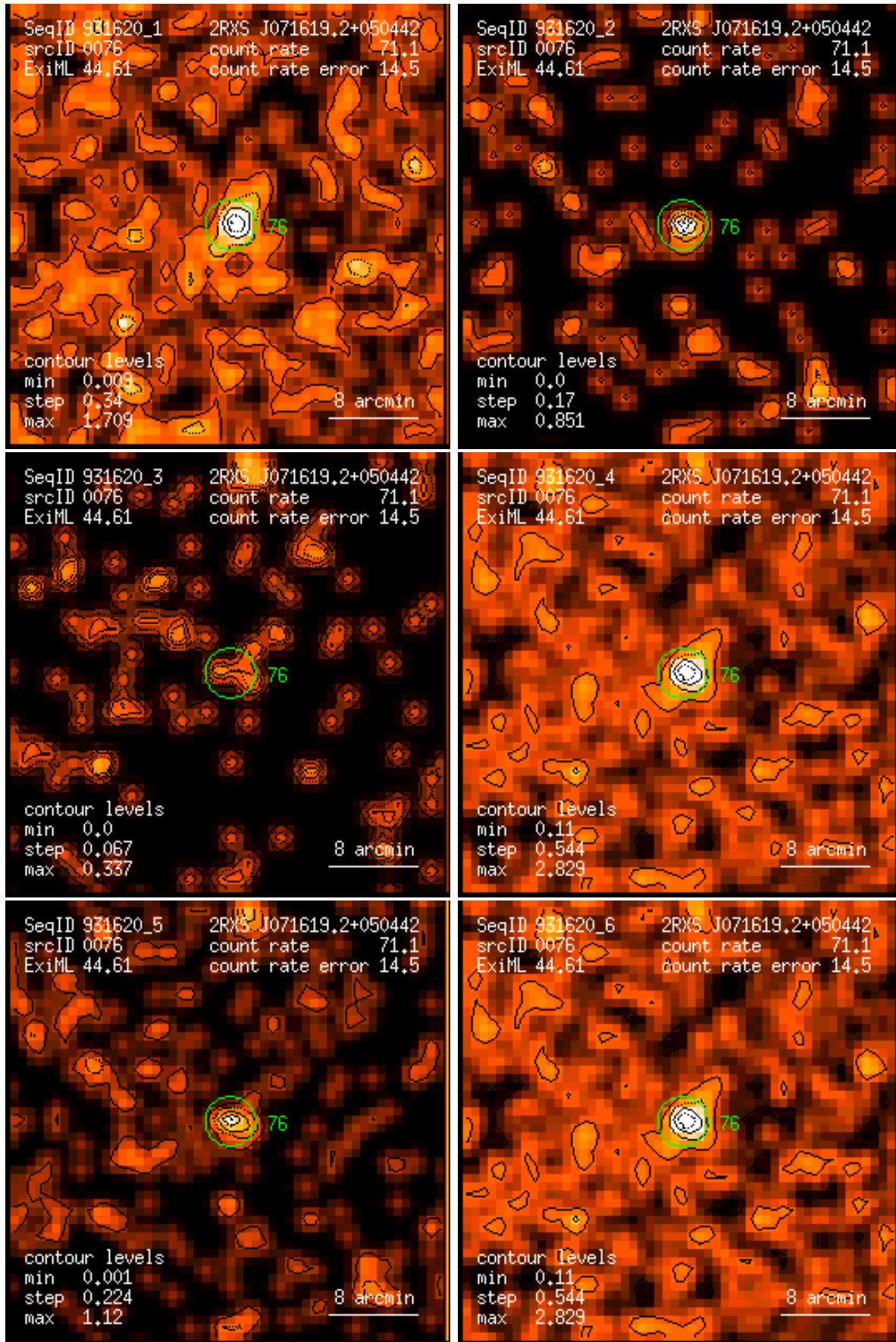
Figure 76: RASS 931620: detection 0076: band rate images, Gaussian filter: (1) PSPC channels 11 – 41, (2) 52 – 90, (3) 91 – 201, (4) 11 – 235, (5) 52 – 201, (6) 11 – 201. Broad band rates in counts/ks. Band rate contour levels in counts/ks/arcmin 2 .
