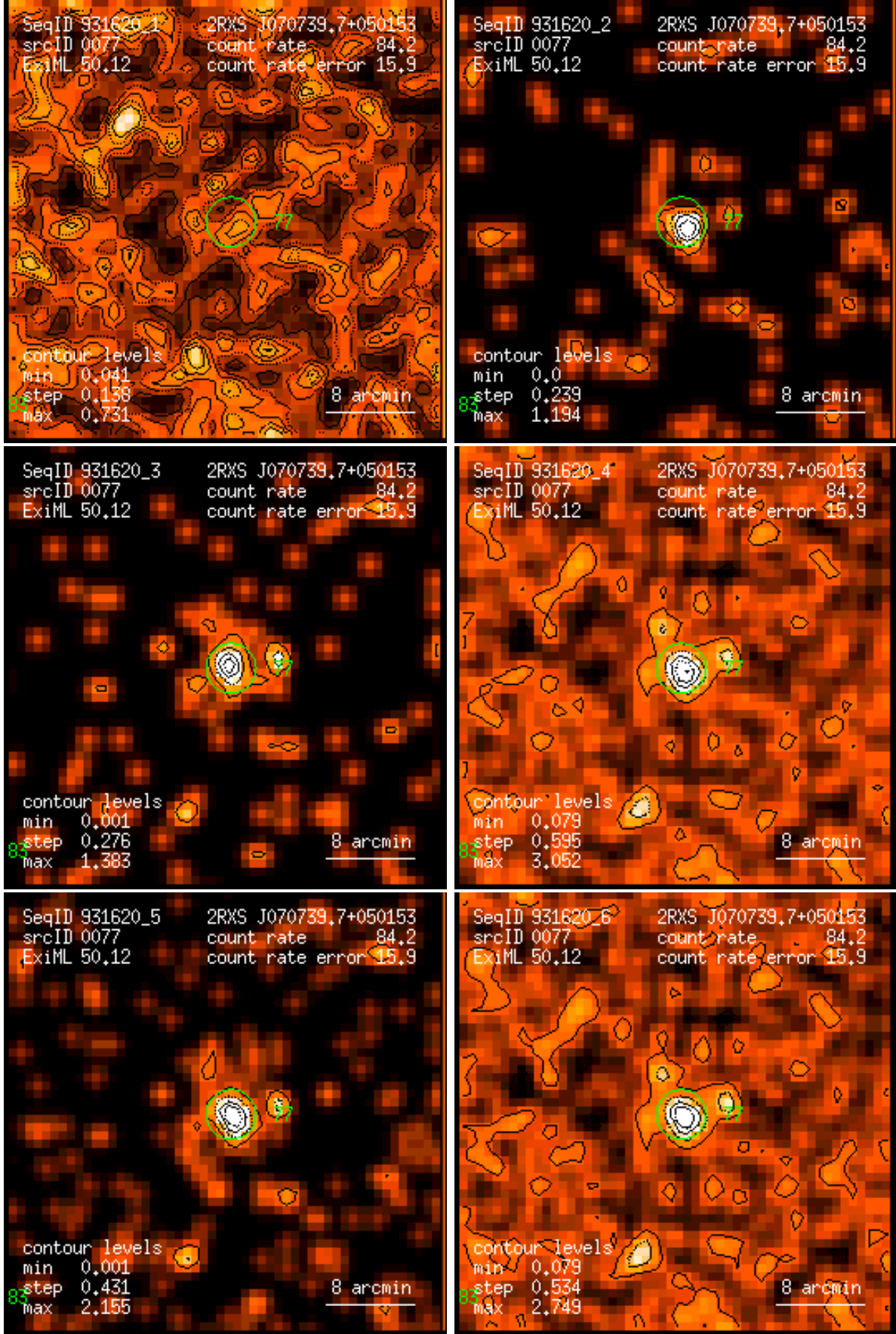
Figure 77: RASS 931620: detection 0077: band rate images, Gaussian filter: (1) PSPC channels 11 – 41, (2) 52 – 90, (3) 91 – 201, (4) 11 – 235, (5) 52 – 201, (6) 11 – 201. Broad band rates in counts/ks. Band rate contour levels in counts/ks/arcmin 2 .
