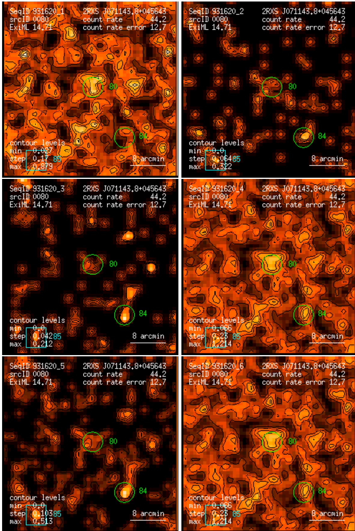
Figure 80: RASS 931620: detection 0080: band rate images, Gaussian filter: (1) PSPC channels 11 – 41, (2) 52 – 90, (3) 91 – 201, (4) 11 – 235, (5) 52 – 201, (6) 11 – 201. Broad band rates in counts/ks. Band rate contour levels in counts/ks/arcmin 2 .
