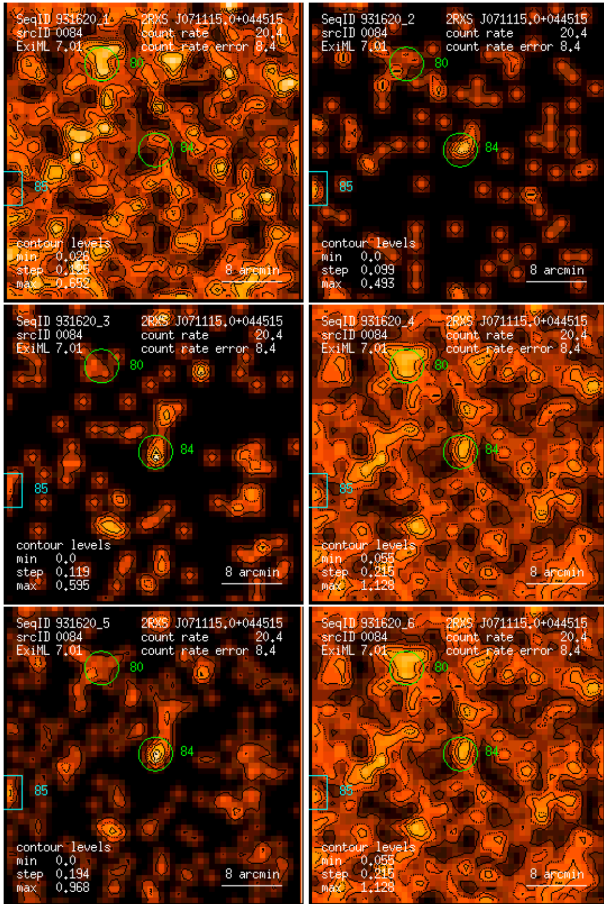
Figure 84: RASS 931620: detection 0084: band rate images, Gaussian filter: (1) PSPC channels 11 – 41, (2) 52 – 90, (3) 91 – 201, (4) 11 – 235, (5) 52 – 201, (6) 11 – 201. Broad band rates in counts/ks. Band rate contour levels in counts/ks/arcmin 2 .
