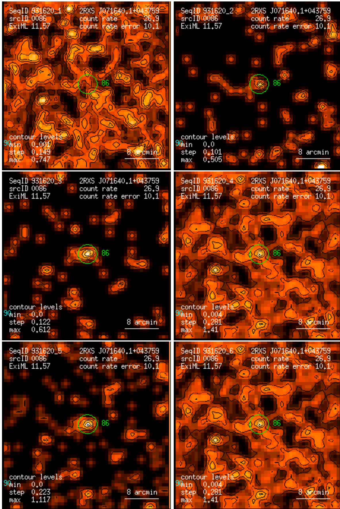
Figure 86: RASS 931620: detection 0086: band rate images, Gaussian filter: (1) PSPC channels 11 – 41, (2) 52 – 90, (3) 91 – 201, (4) 11 – 235, (5) 52 – 201, (6) 11 – 201. Broad band rates in counts/ks. Band rate contour levels in counts/ks/arcmin 2 .
