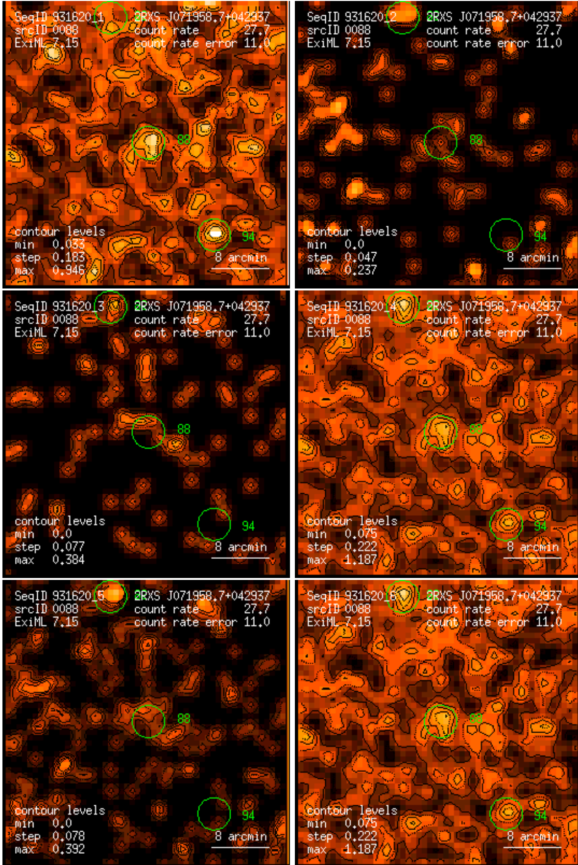
Figure 88: RASS 931620: detection 0088: band rate images, Gaussian filter: (1) PSPC channels 11 – 41, (2) 52 – 90, (3) 91 – 201, (4) 11 – 235, (5) 52 – 201, (6) 11 – 201. Broad band rates in counts/ks. Band rate contour levels in counts/ks/arcmin 2 .
