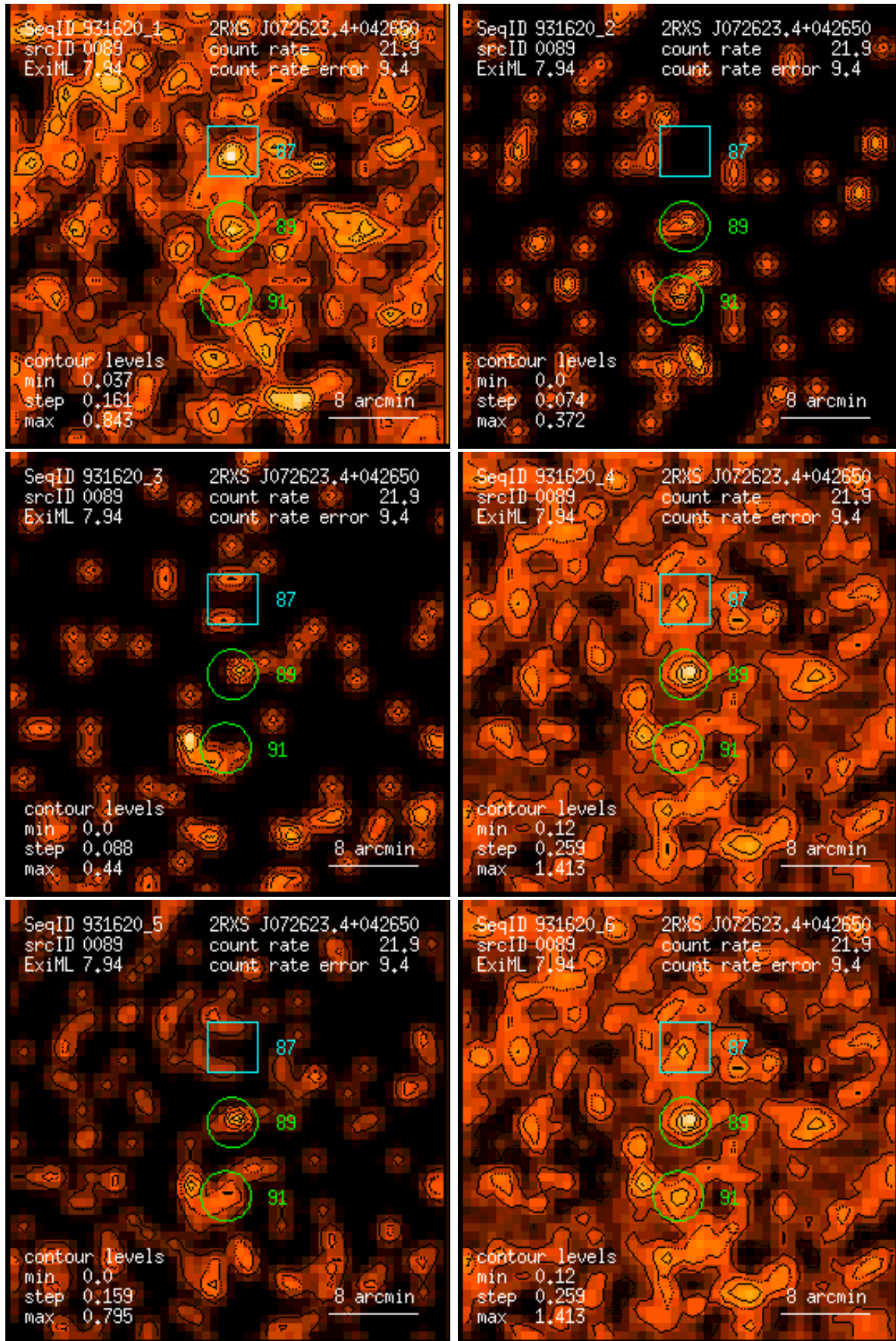
Figure 89: RASS 931620: detection 0089: band rate images, Gaussian filter: (1) PSPC channels 11 – 41, (2) 52 – 90, (3) 91 – 201, (4) 11 – 235, (5) 52 – 201, (6) 11 – 201. Broad band rates in counts/ks. Band rate contour levels in counts/ks/arcmin 2 .
