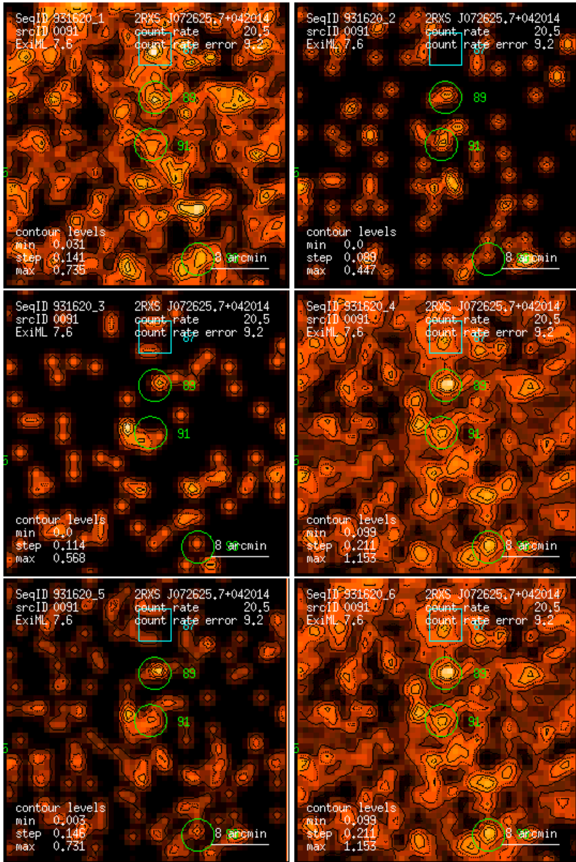
Figure 91: RASS 931620: detection 0091: band rate images, Gaussian filter: (1) PSPC channels 11 – 41, (2) 52 – 90, (3) 91 – 201, (4) 11 – 235, (5) 52 – 201, (6) 11 – 201. Broad band rates in counts/ks. Band rate contour levels in counts/ks/arcmin 2 .
