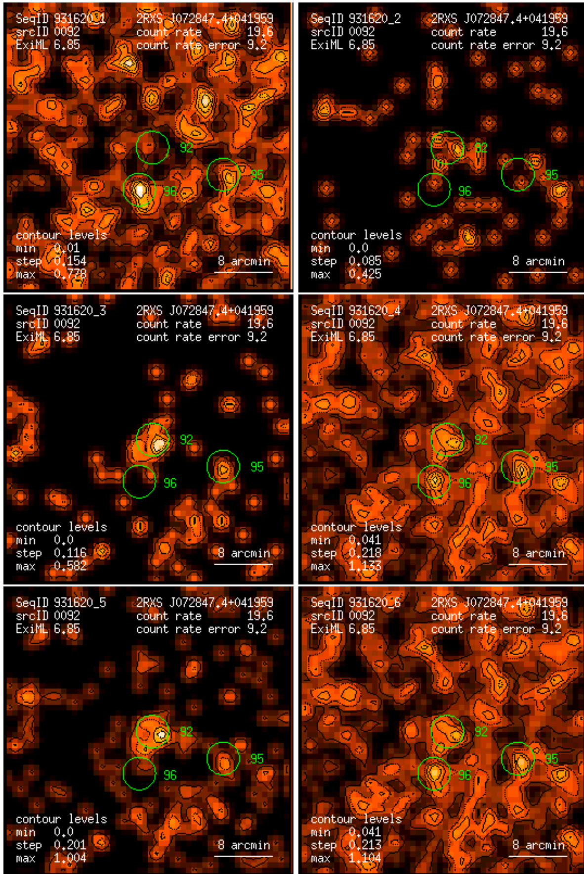
Figure 92: RASS 931620: detection 0092: band rate images, Gaussian filter: (1) PSPC channels 11 – 41, (2) 52 – 90, (3) 91 – 201, (4) 11 – 235, (5) 52 – 201, (6) 11 – 201. Broad band rates in counts/ks. Band rate contour levels in counts/ks/arcmin 2 .
