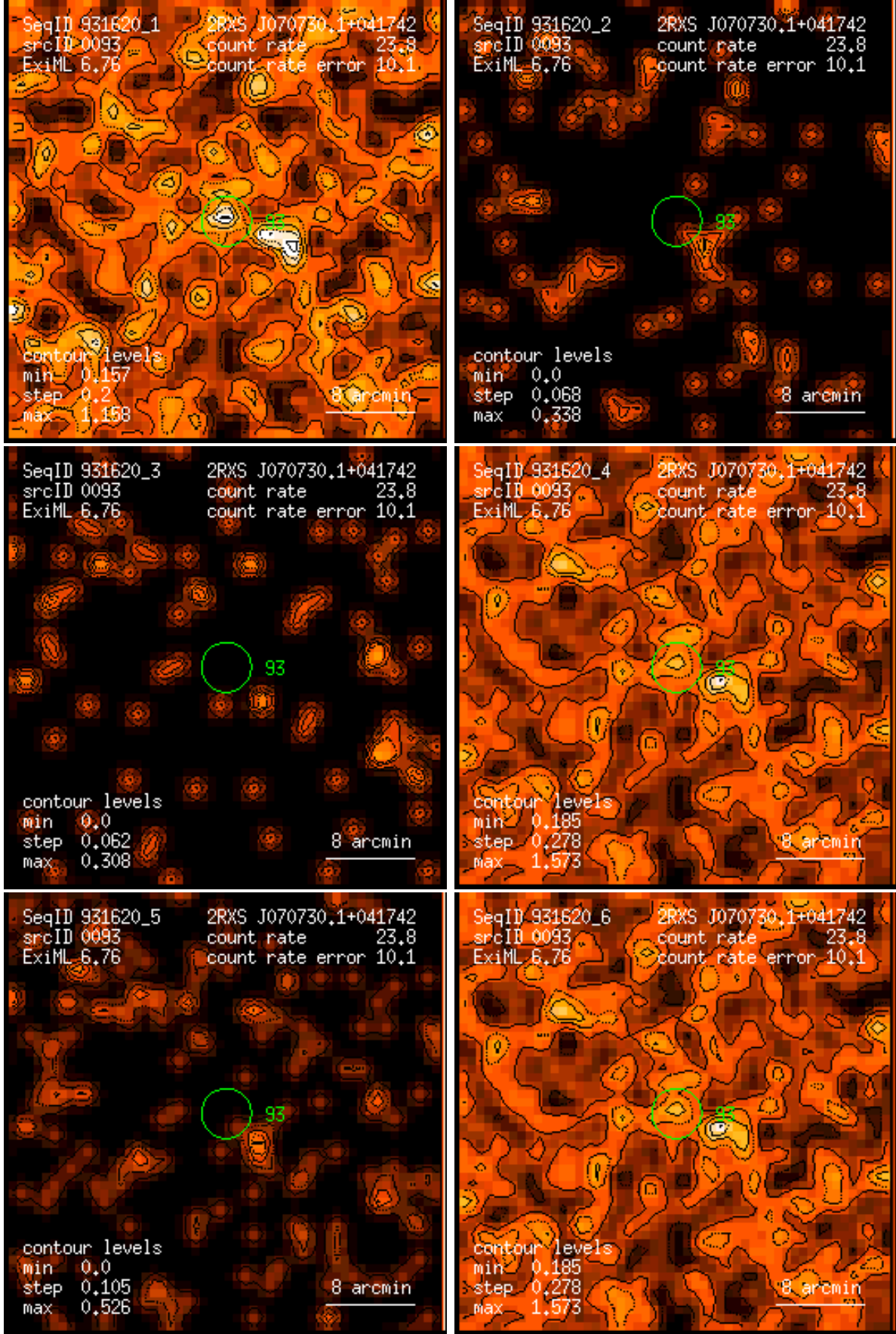
Figure 93: RASS 931620: detection 0093: band rate images, Gaussian filter: (1) PSPC channels 11 – 41, (2) 52 – 90, (3) 91 – 201, (4) 11 – 235, (5) 52 – 201, (6) 11 – 201. Broad band rates in counts/ks. Band rate contour levels in counts/ks/arcmin 2 .
