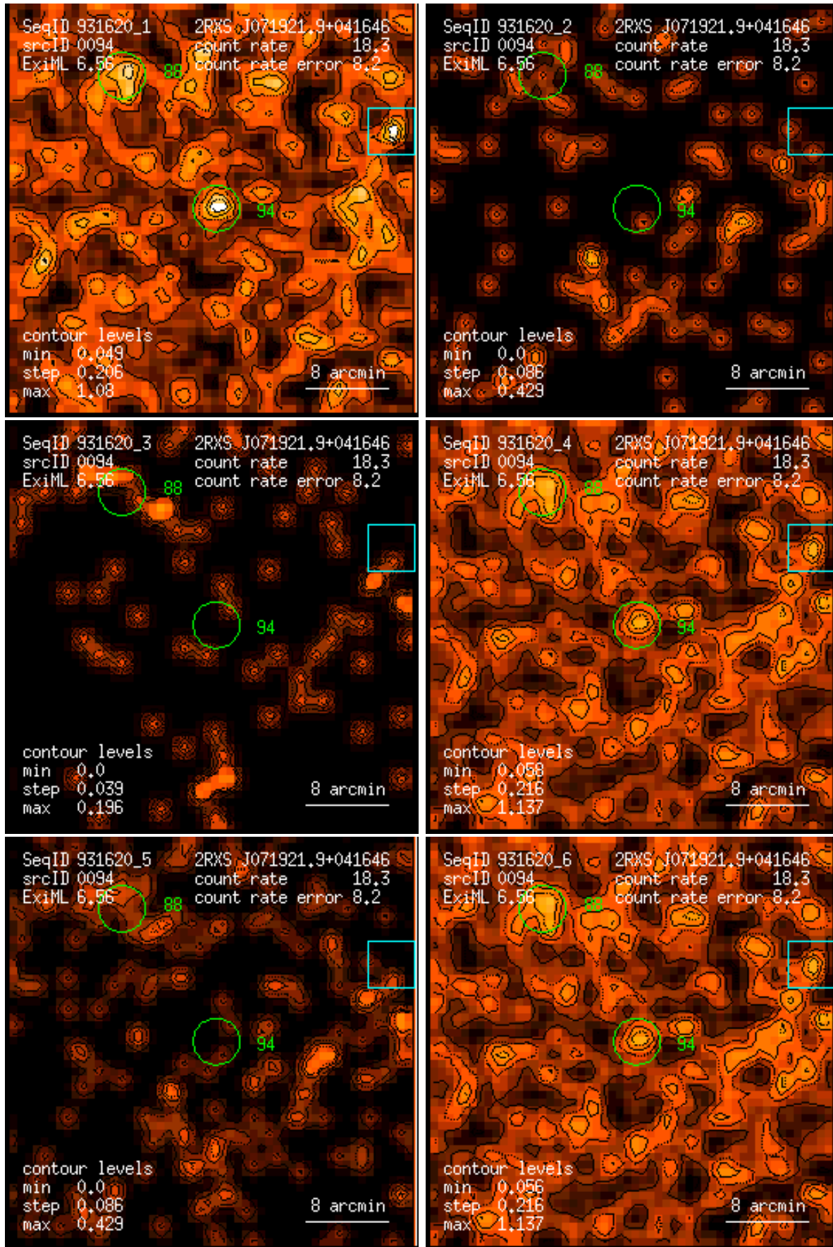
Figure 94: RASS 931620: detection 0094: band rate images, Gaussian filter: (1) PSPC channels 11 – 41, (2) 52 – 90, (3) 91 – 201, (4) 11 – 235, (5) 52 – 201, (6) 11 – 201. Broad band rates in counts/ks. Band rate contour levels in counts/ks/arcmin 2 .
