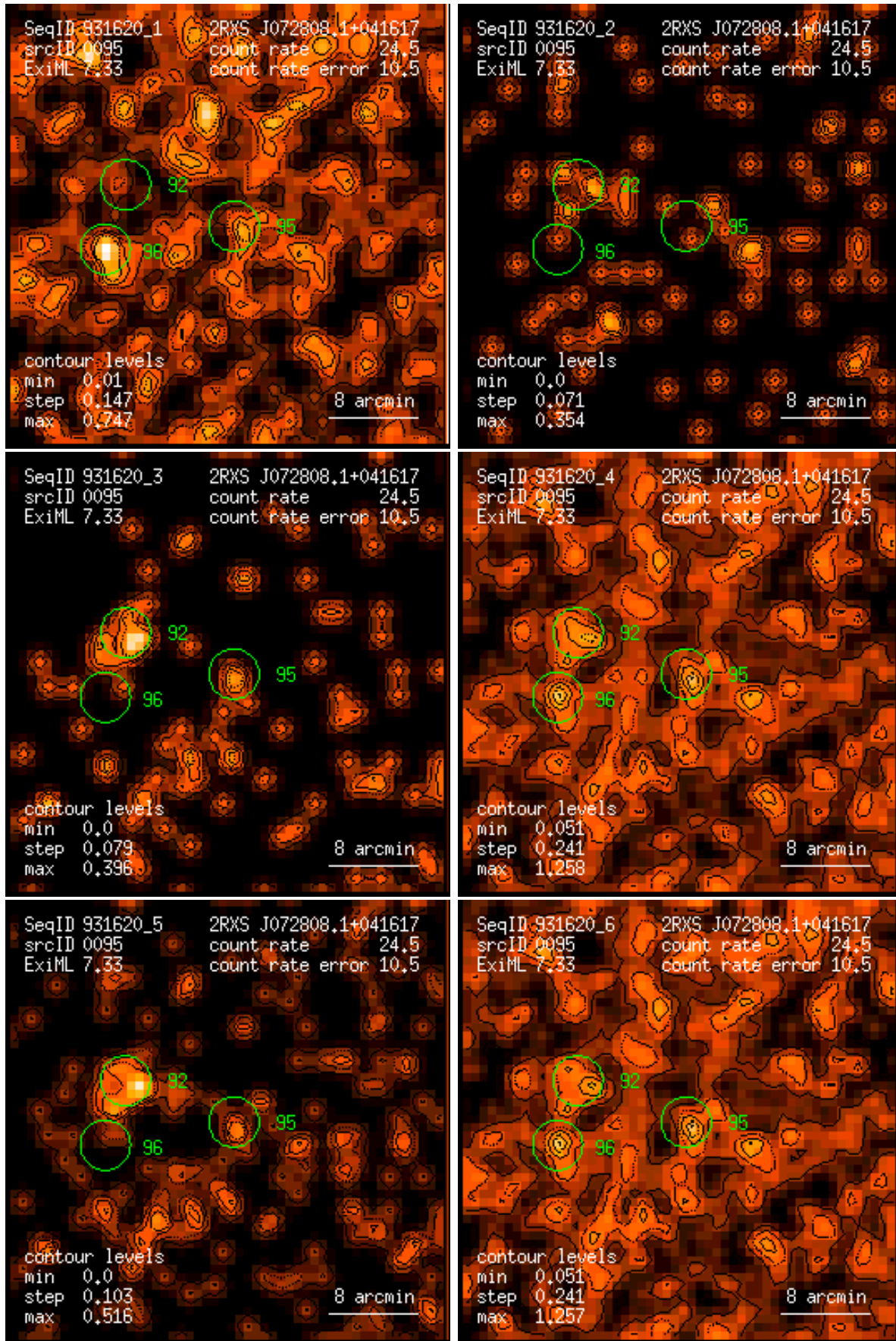
Figure 95: RASS 931620: detection 0095: band rate images, Gaussian filter: (1) PSPC channels 11 – 41, (2) 52 – 90, (3) 91 – 201, (4) 11 – 235, (5) 52 – 201, (6) 11 – 201. Broad band rates in counts/ks. Band rate contour levels in counts/ks/arcmin 2 .
