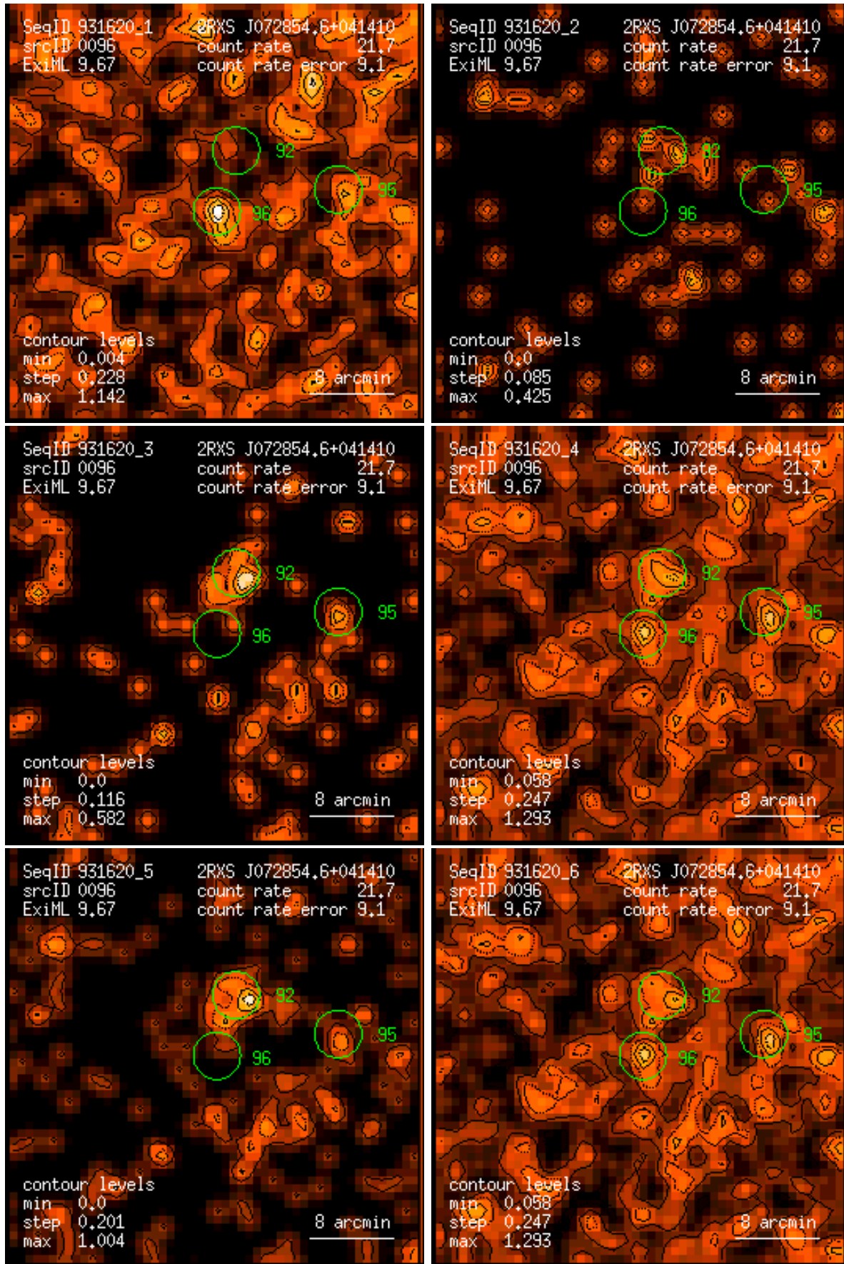
Figure 96: RASS 931620: detection 0096: band rate images, Gaussian filter: (1) PSPC channels 11 – 41, (2) 52 – 90, (3) 91 – 201, (4) 11 – 235, (5) 52 – 201, (6) 11 – 201. Broad band rates in counts/ks. Band rate contour levels in counts/ks/arcmin 2 .
