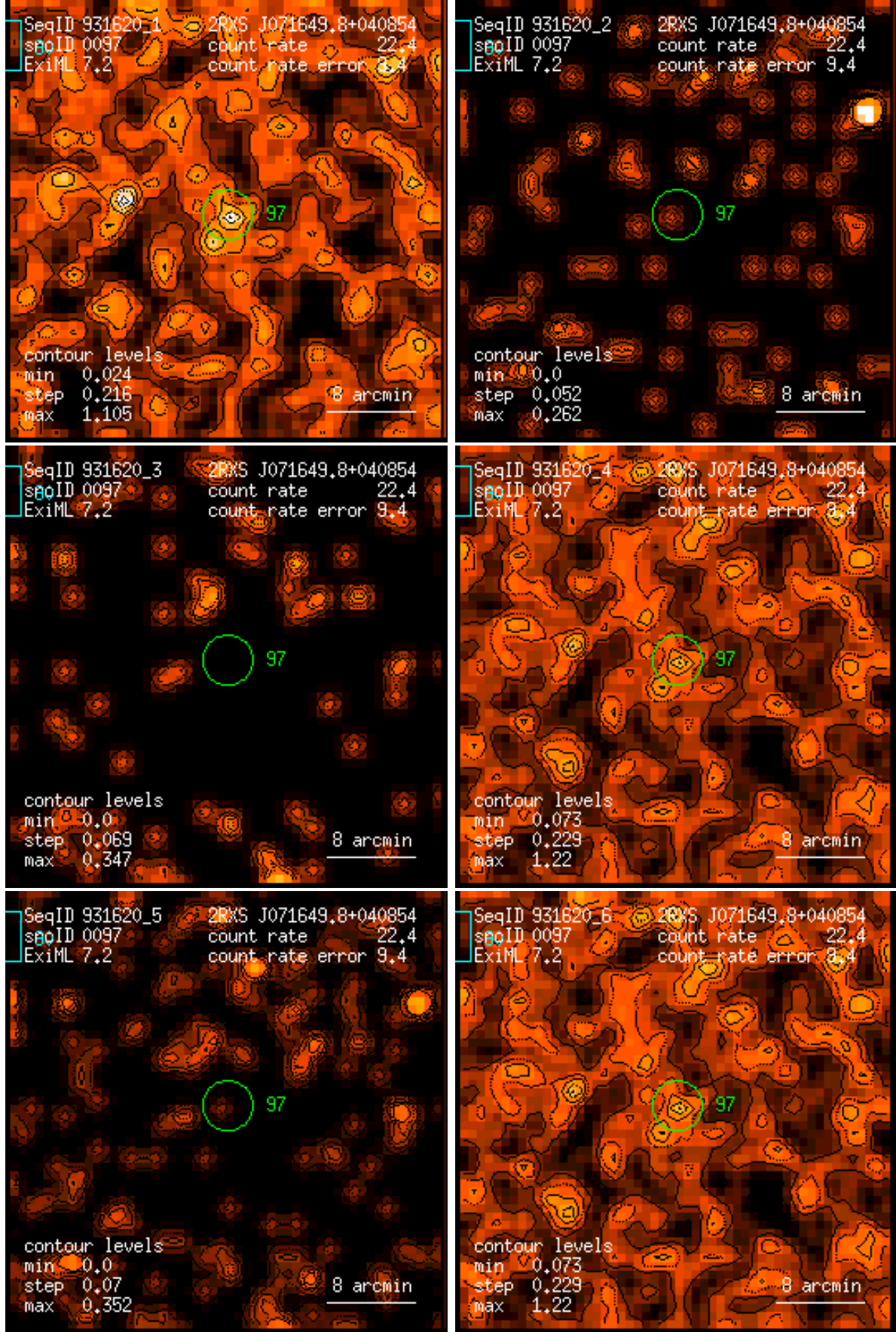
Figure 97: RASS 931620: detection 0097: band rate images, Gaussian filter: (1) PSPC channels 11 – 41, (2) 52 – 90, (3) 91 – 201, (4) 11 – 235, (5) 52 – 201, (6) 11 – 201. Broad band rates in counts/ks. Band rate contour levels in counts/ks/arcmin 2 .
