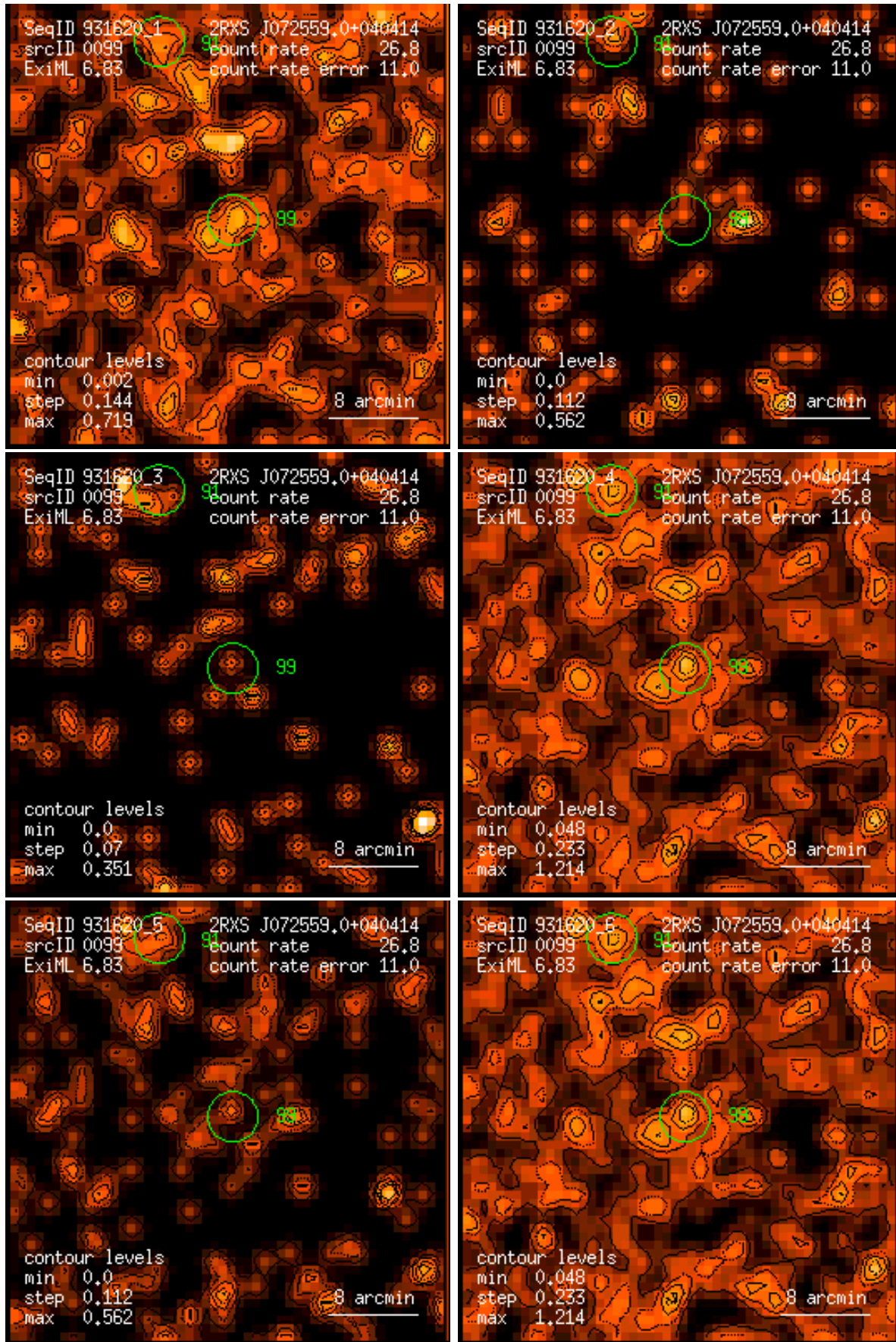
Figure 99: RASS 931620: detection 0099: band rate images, Gaussian filter: (1) PSPC channels 11 – 41, (2) 52 – 90, (3) 91 – 201, (4) 11 – 235, (5) 52 – 201, (6) 11 – 201. Broad band rates in counts/ks. Band rate contour levels in counts/ks/arcmin 2 .
