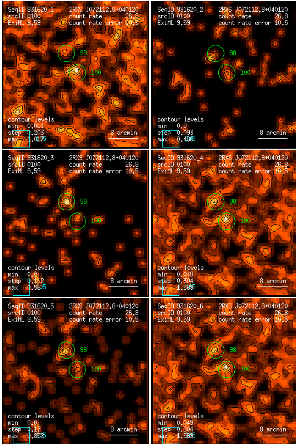
Figure 100: RASS 931620: detection 0100: band rate images, Gaussian filter: (1) PSPC channels 11 – 41, (2) 52 – 90, (3) 91 – 201, (4) 11 – 235, (5) 52 – 201, (6) 11 – 201. Broad band rates in counts/ks. Band rate contour levels in counts/ks/arcmin 2 .
