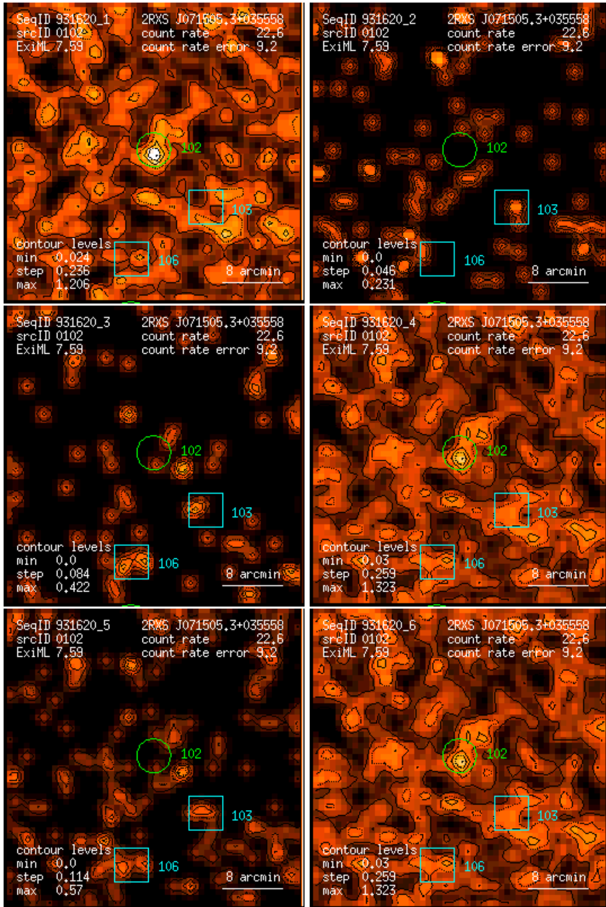
Figure 102: RASS 931620: detection 0102: band rate images, Gaussian filter: (1) PSPC channels 11 – 41, (2) 52 – 90, (3) 91 – 201, (4) 11 – 235, (5) 52 – 201, (6) 11 – 201. Broad band rates in counts/ks. Band rate contour levels in counts/ks/arcmin 2 .
