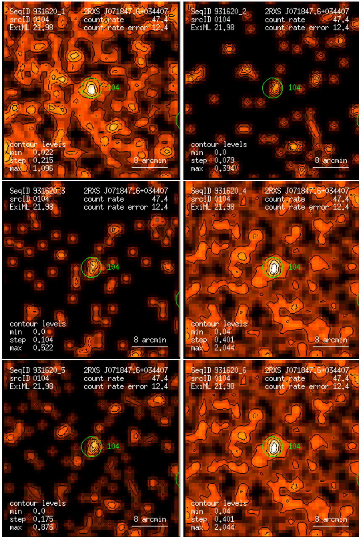
Figure 104: RASS 931620: detection 0104: band rate images, Gaussian filter: (1) PSPC channels 11 – 41, (2) 52 – 90, (3) 91 – 201, (4) 11 – 235, (5) 52 – 201, (6) 11 – 201. Broad band rates in counts/ks. Band rate contour levels in counts/ks/arcmin 2 .
