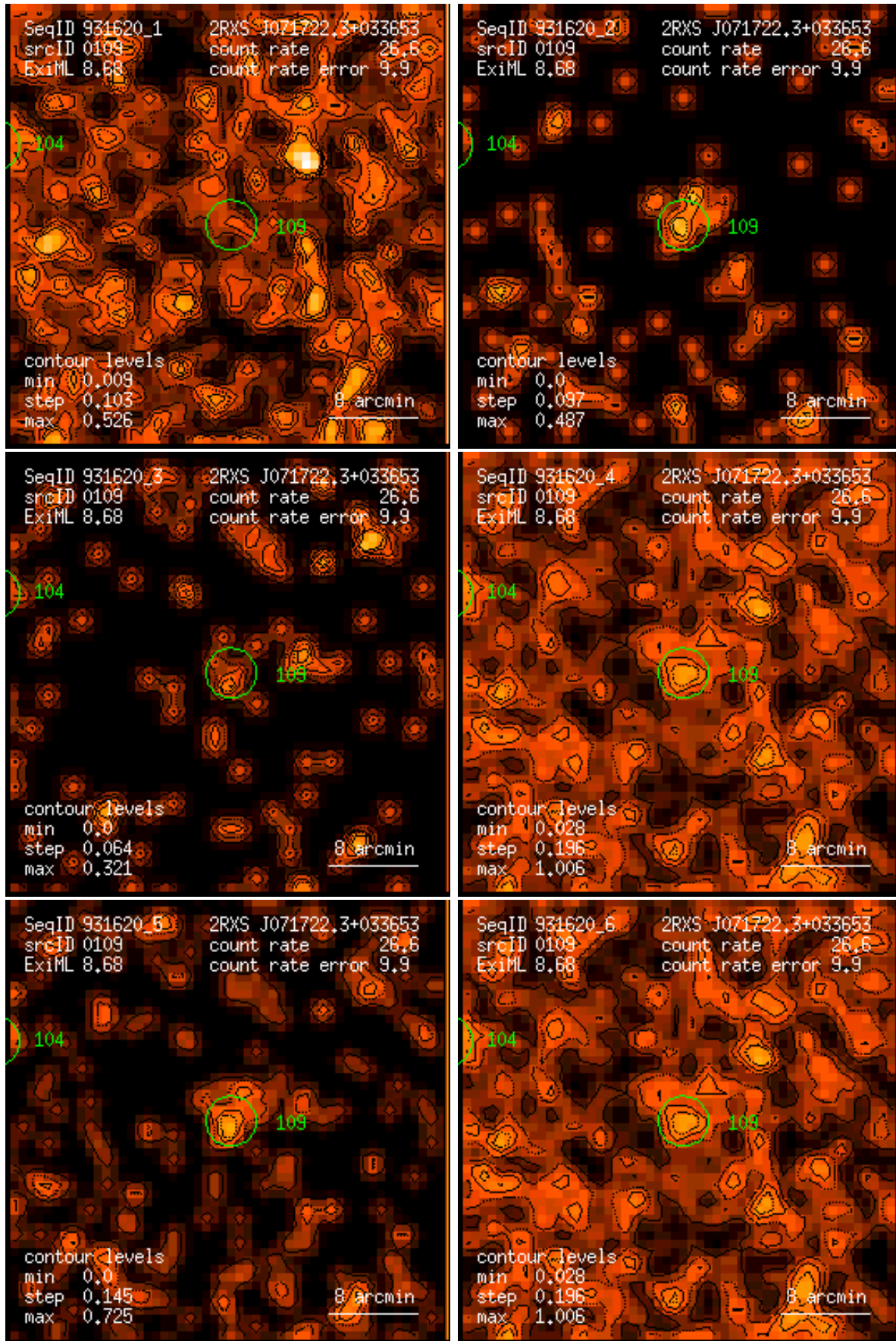
Figure 109: RASS 931620: detection 0109: band rate images, Gaussian filter: (1) PSPC channels 11 – 41, (2) 52 – 90, (3) 91 – 201, (4) 11 – 235, (5) 52 – 201, (6) 11 – 201. Broad band rates in counts/ks. Band rate contour levels in counts/ks/arcmin 2 .
