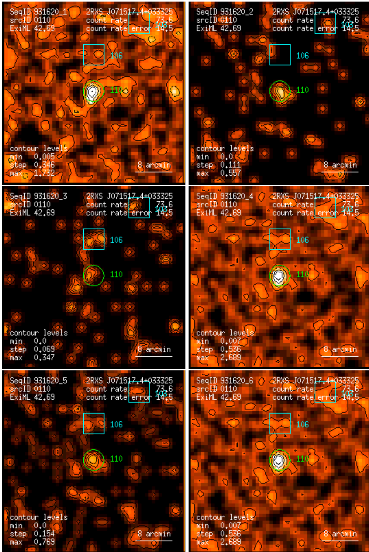
Figure 110: RASS 931620: detection 0110: band rate images, Gaussian filter: (1) PSPC channels 11 – 41, (2) 52 – 90, (3) 91 – 201, (4) 11 – 235, (5) 52 – 201, (6) 11 – 201. Broad band rates in counts/ks. Band rate contour levels in counts/ks/arcmin 2 .
