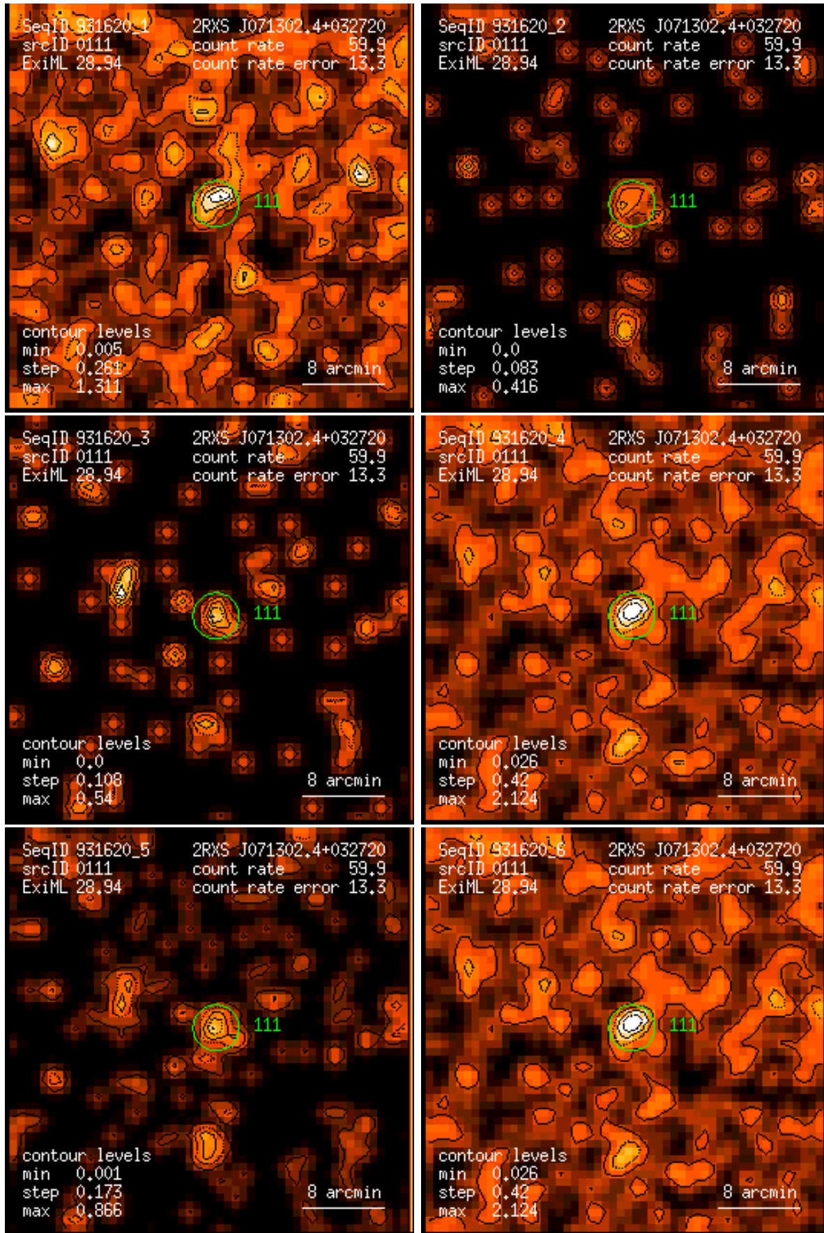
Figure 111: RASS 931620: detection 0111: band rate images, Gaussian filter: (1) PSPC channels 11 – 41, (2) 52 – 90, (3) 91 – 201, (4) 11 – 235, (5) 52 – 201, (6) 11 – 201. Broad band rates in counts/ks. Band rate contour levels in counts/ks/arcmin 2 .
