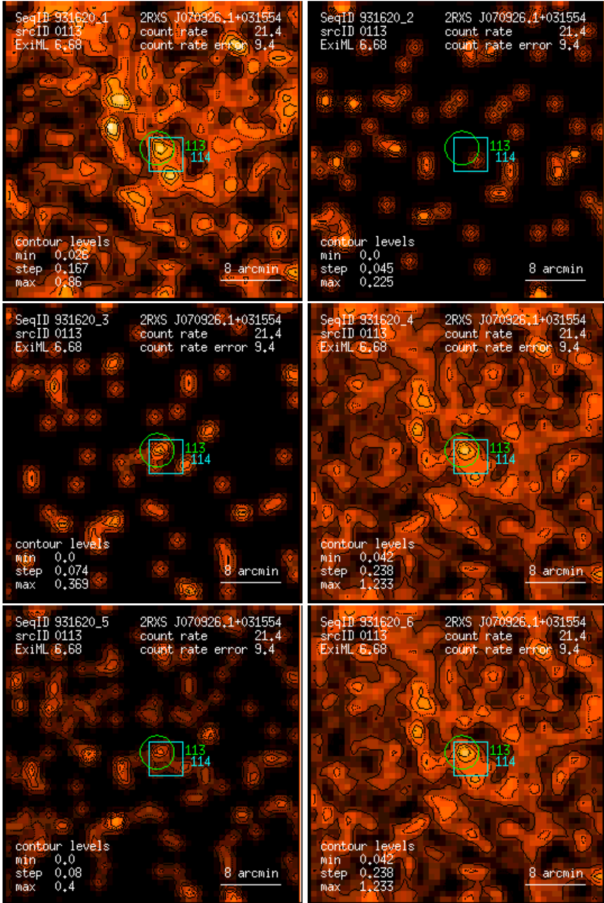
Figure 113: RASS 931620: detection 0113: band rate images, Gaussian filter: (1) PSPC channels 11 – 41, (2) 52 – 90, (3) 91 – 201, (4) 11 – 235, (5) 52 – 201, (6) 11 – 201. Broad band rates in counts/ks. Band rate contour levels in counts/ks/arcmin 2 .
