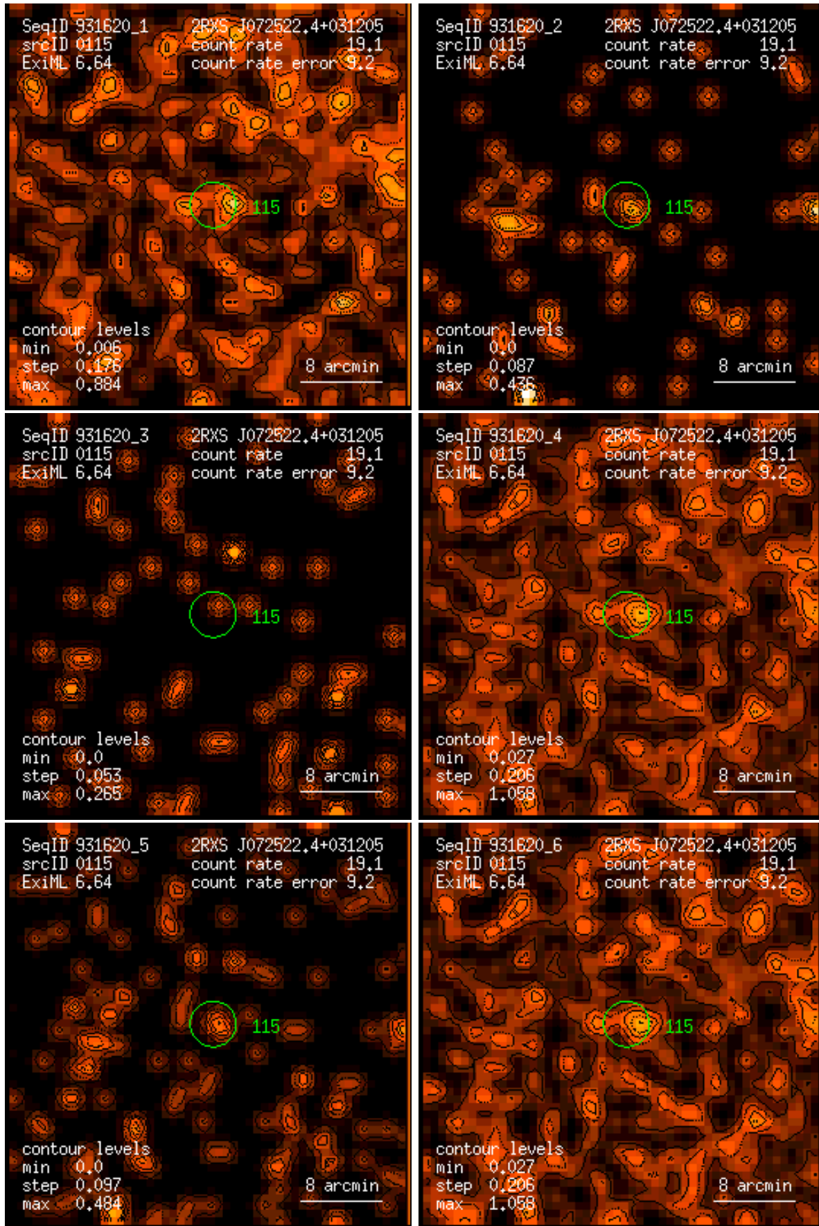
Figure 115: RASS 931620: detection 0115: band rate images, Gaussian filter: (1) PSPC channels 11 – 41, (2) 52 – 90, (3) 91 – 201, (4) 11 – 235, (5) 52 – 201, (6) 11 – 201. Broad band rates in counts/ks. Band rate contour levels in counts/ks/arcmin 2 .
