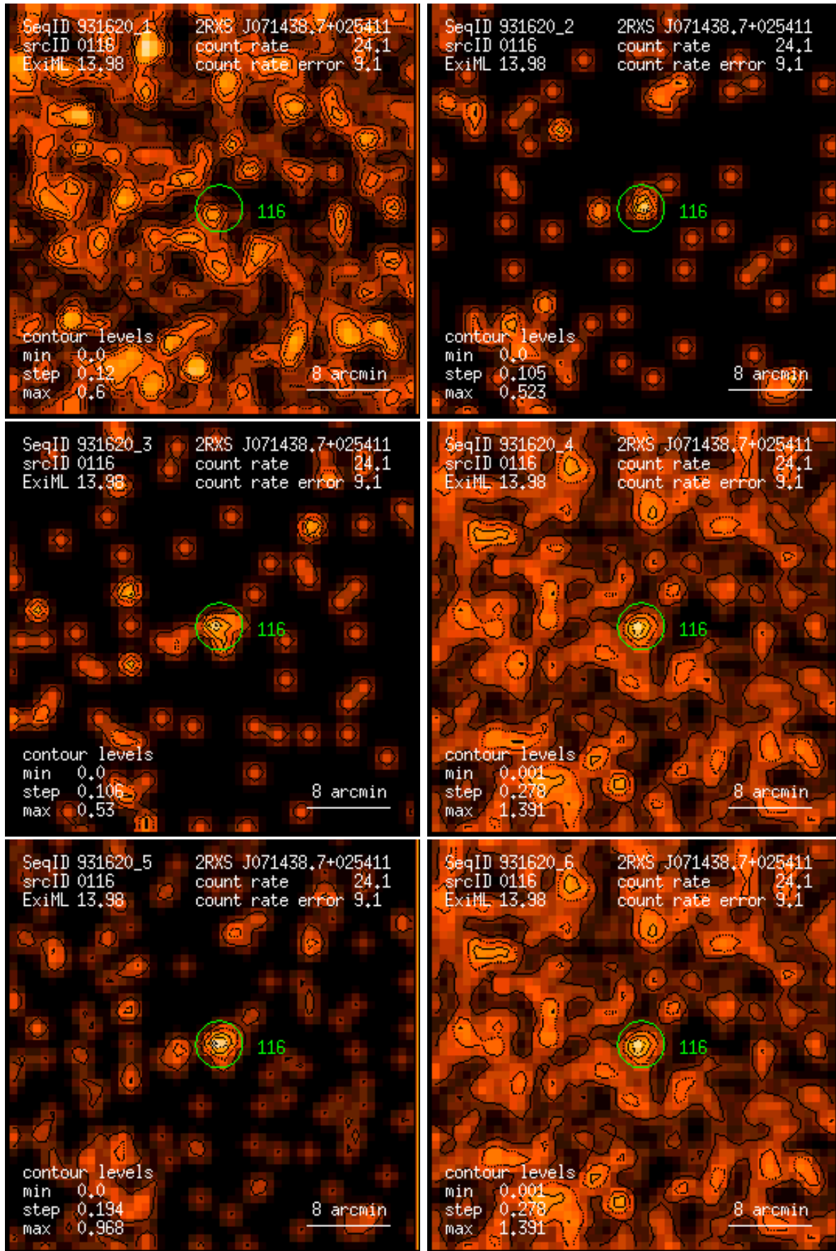
Figure 116: RASS 931620: detection 0116: band rate images, Gaussian filter: (1) PSPC channels 11 – 41, (2) 52 – 90, (3) 91 – 201, (4) 11 – 235, (5) 52 – 201, (6) 11 – 201. Broad band rates in counts/ks. Band rate contour levels in counts/ks/arcmin 2 .
