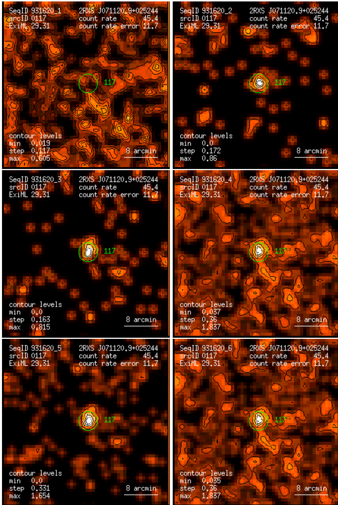
Figure 117: RASS 931620: detection 0117: band rate images, Gaussian filter: (1) PSPC channels 11 – 41, (2) 52 – 90, (3) 91 – 201, (4) 11 – 235, (5) 52 – 201, (6) 11 – 201. Broad band rates in counts/ks. Band rate contour levels in counts/ks/arcmin 2 .
