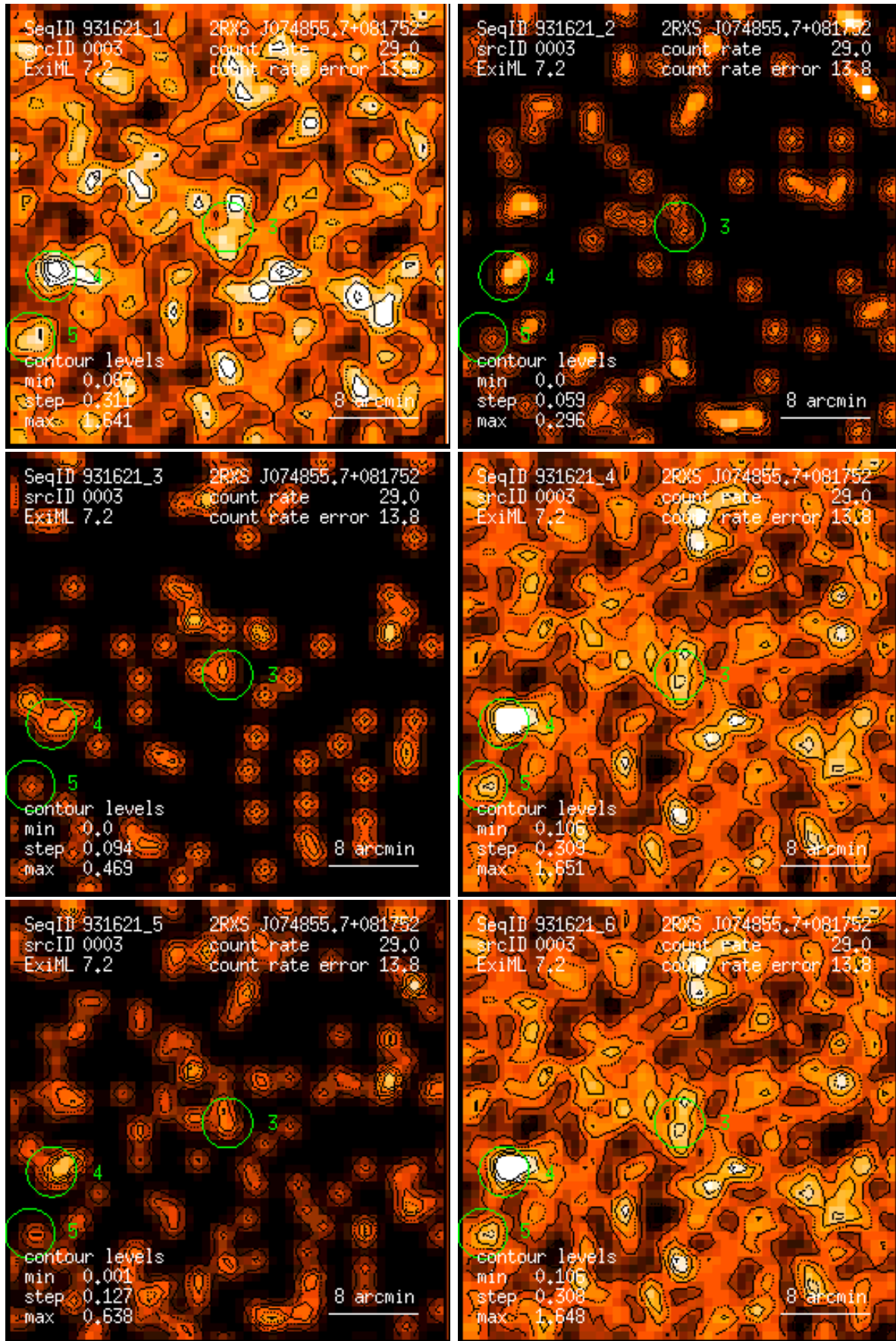
Figure 3: RASS 931621: detection 0003: band rate images, Gaussian filter: (1) PSPC channels 11 – 41, (2) 52 – 90, (3) 91 – 201, (4) 11 – 235, (5) 52 – 201, (6) 11 – 201. Broad band rates in counts/ks. Band rate contour levels in counts/ks/arcmin 2 .
