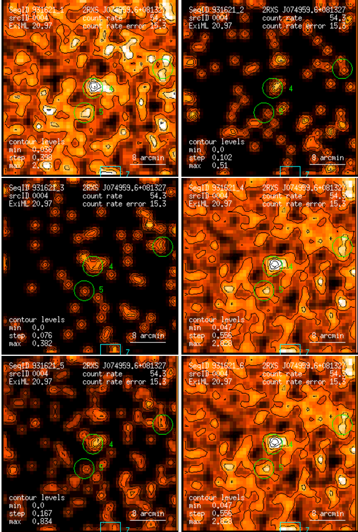
Figure 4: RASS 931621: detection 0004: band rate images, Gaussian filter: (1) PSPC channels 11 – 41, (2) 52 – 90, (3) 91 – 201, (4) 11 – 235, (5) 52 – 201, (6) 11 – 201. Broad band rates in counts/ks. Band rate contour levels in counts/ks/arcmin 2 .
